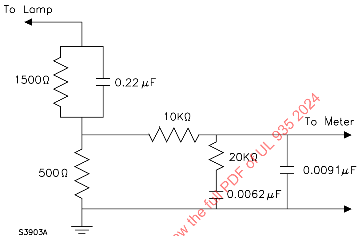
Figure 24.2 Alternative circuit – through lamp
