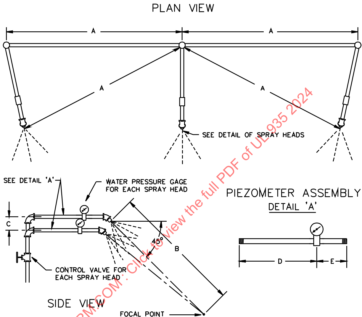
Figure 37.2 Spray head pipe rack
