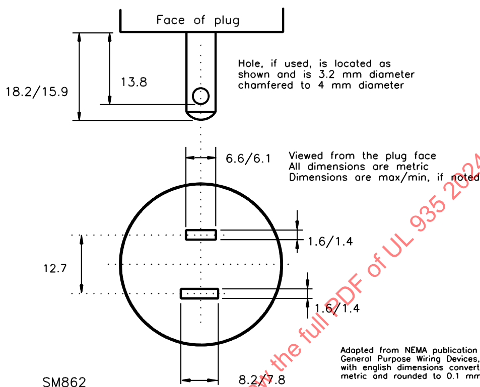
Figure 13.2 Polarized plug dimensions
