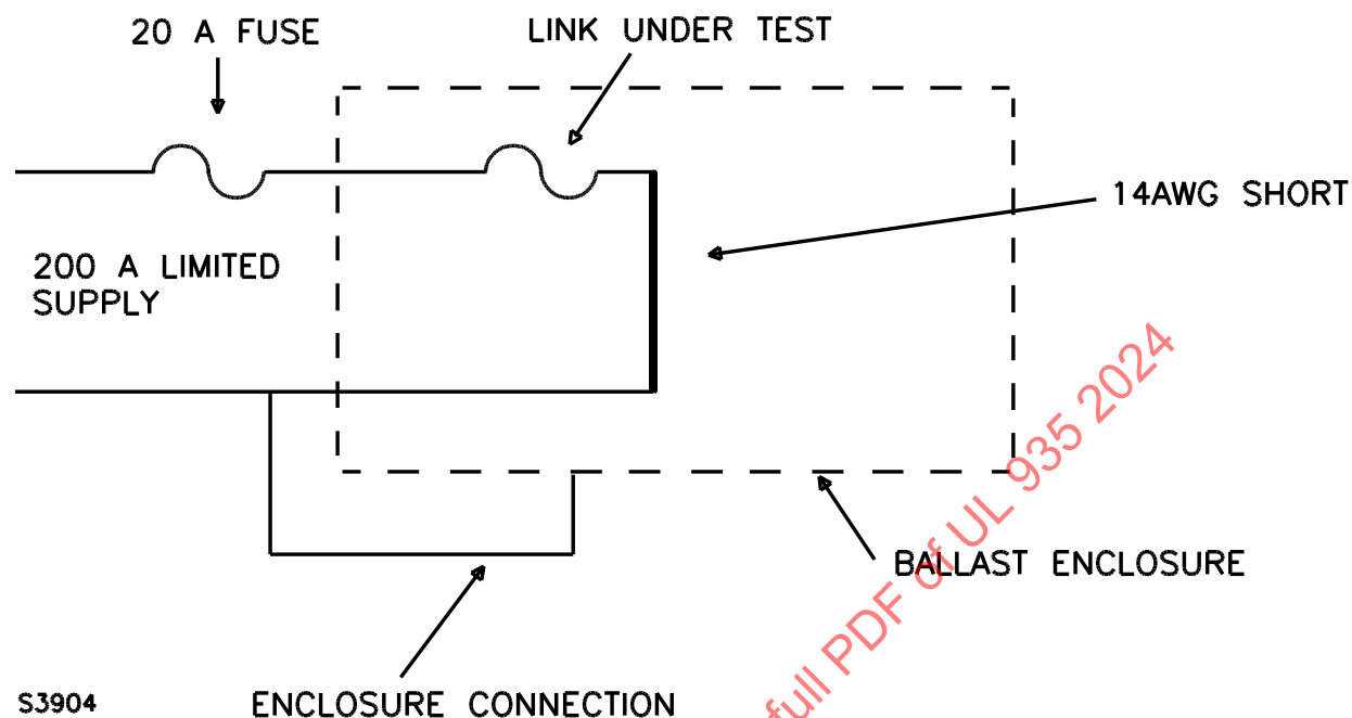
Figure 34.1 Connection for paragraph 34.2
