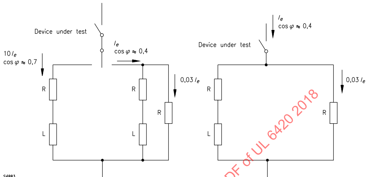
Figure 9.1 AC test circuits (see Clause 9.1.2.4.2.5)
