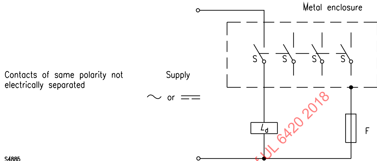
Figure 9.4 Test circuits for multi-pole control switches – Contacts of same polarity, not electrically separated
