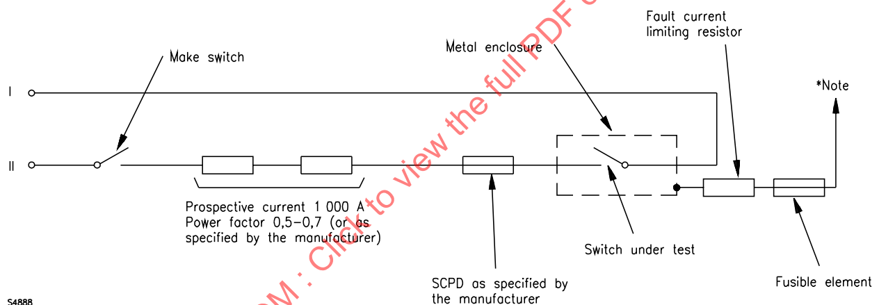
Figure 9.8 Test circuit, conditional short-circuit current
