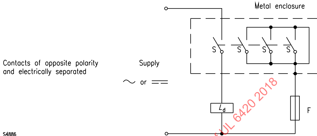
Figure 9.5 Test circuits or multi-pole control switches – contacts of opposite polarity, and not electrically separated
