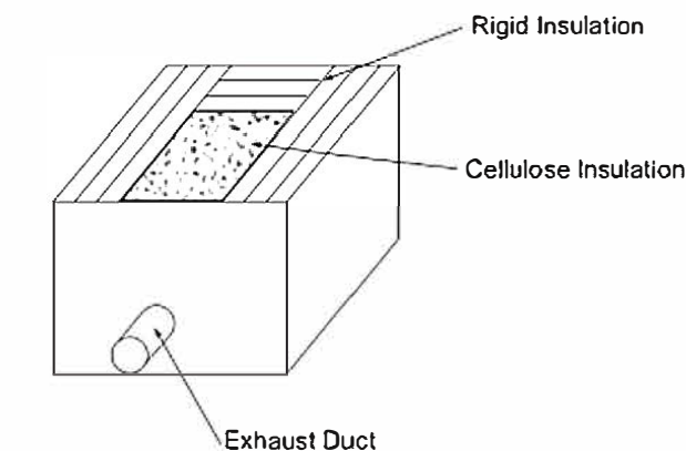
Figure 144.0 Insulation Box Configuration
