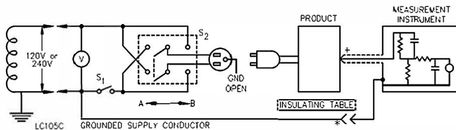
Figure 41.1 Leakage current measurement circuits
