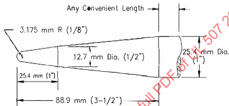
Figure 163.1 Probe for moving parts of floor insert fans
