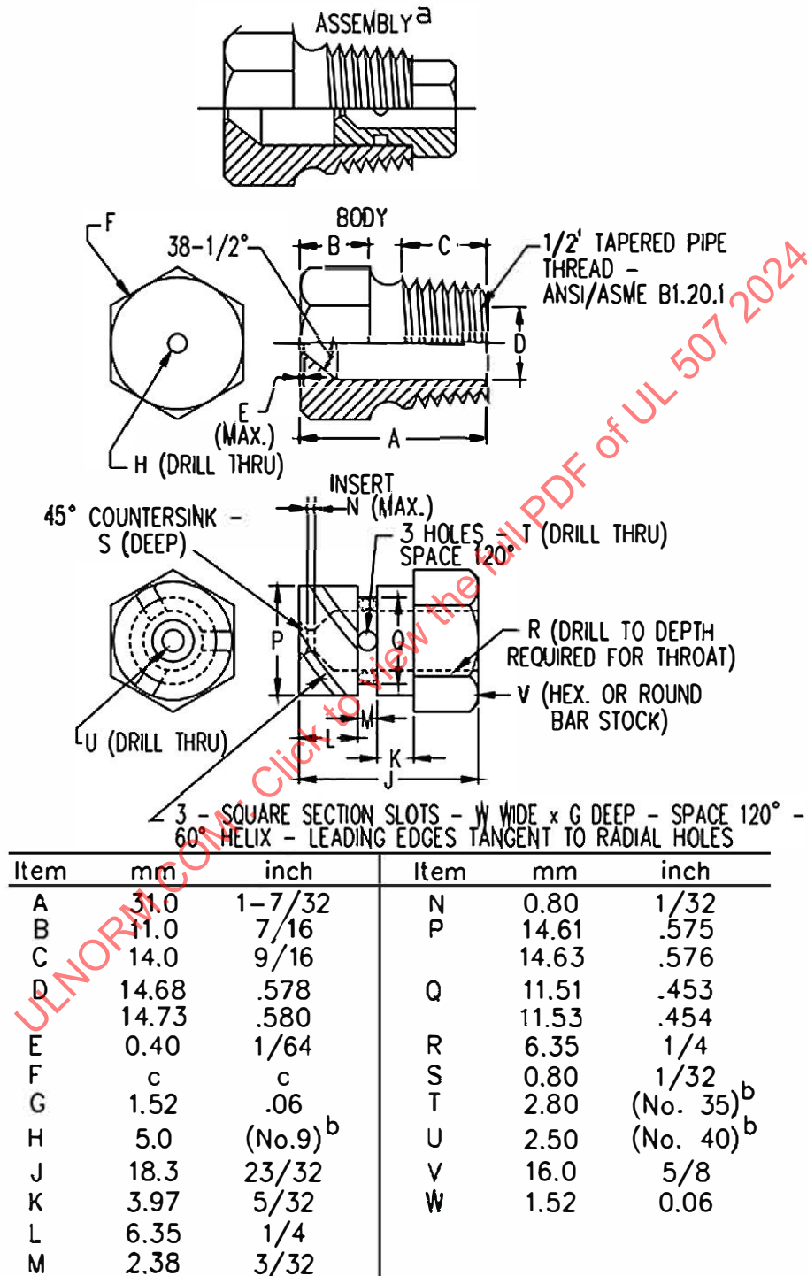
Figure 48.2 Spray head assembly
