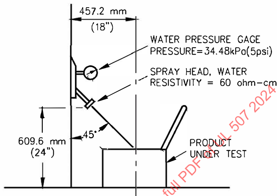
Figure 157.1 Set-up for water spray test
