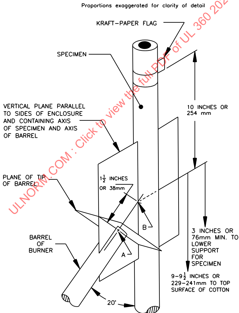
Figure 16.1 Essential dimensions for vertical flame test
