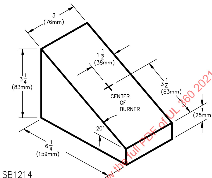
Figure 16.2 Dimensions of wedge in inches (millimeters)
