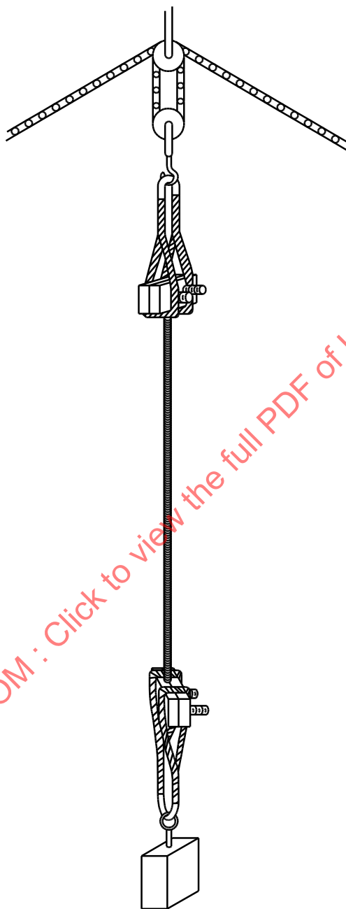
Figure 11.1 Tension test using block and tackle
