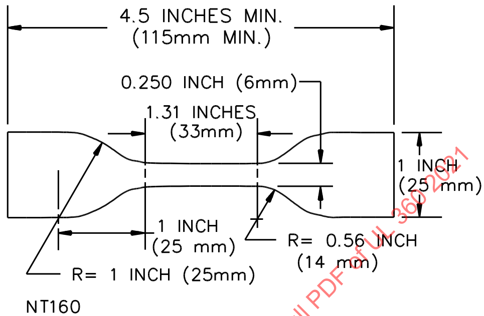
Figure 17.1 Die for cutting specimens
