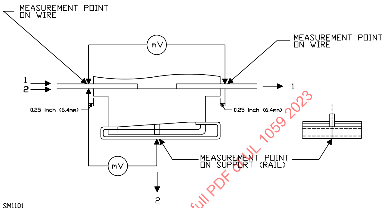
Figure 50.1 Voltage drop measurement points
