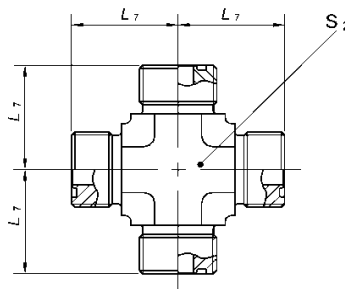
FIGURE 32 - UNION CROSS (52M0501)
