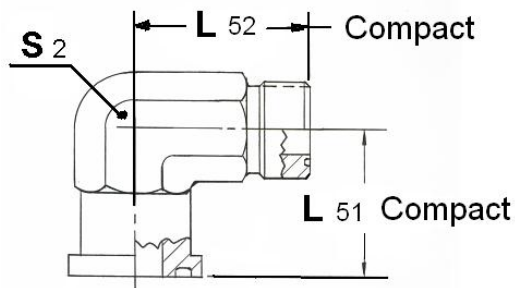
FIGURE 46A (COMPACT – 52M3461 OR 52M3462)
