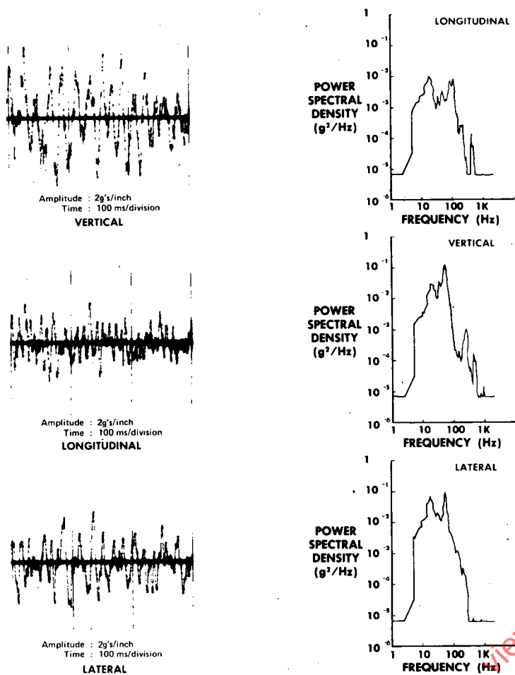
FIG. 14—FRAME TRANSMISSION MOUNT VIBRATION MEASUREMENTS
