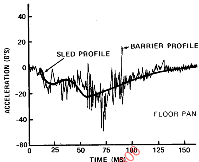
FIG. 6—48 KM/H (30 MPH) BARRIER AND SLED SHOCK PROFILES
