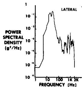
FIG. 13—FRAME BUMPER ATTACHMENT VIBRATION MEASUREMENTS
