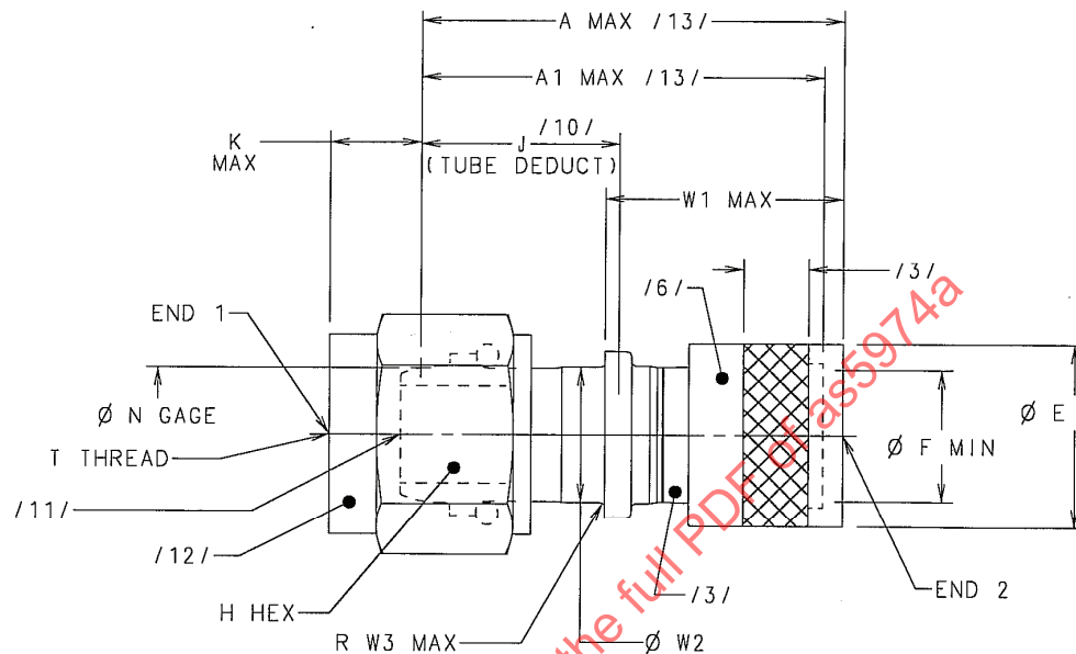
FIGURE 1 ADAPTER, SWAGE
