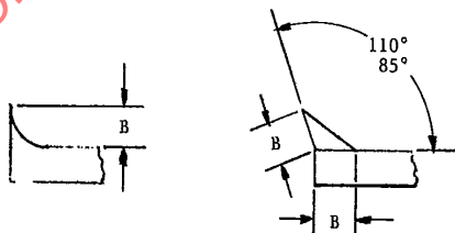
FIG 3 ACCEPTABLE WEDGE CONFIGURATIONS
