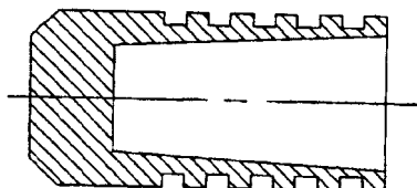
FIGURE 2 - AS3129 PLUG
