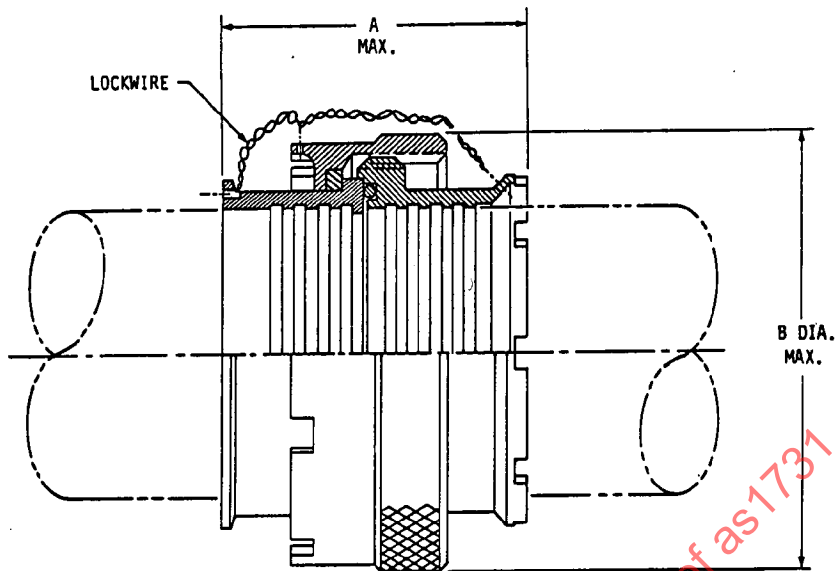
TYPE II COUPLING - ASSEMBLED VIEW
