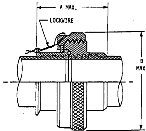
TYPE I COUPLING -ASSEMBLED VIEW
