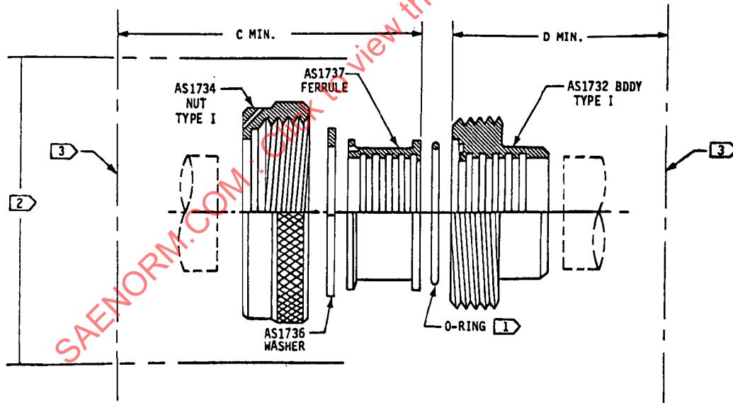
TYPE I COUPLING - EXPLODED VIEW EXPLODED VIEW
