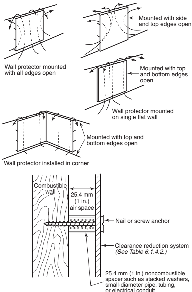
FIGURE 6.1.4.2(a) Sheet Metal or Other Protection to Reduce Required Clearance from Heating Appliance.
