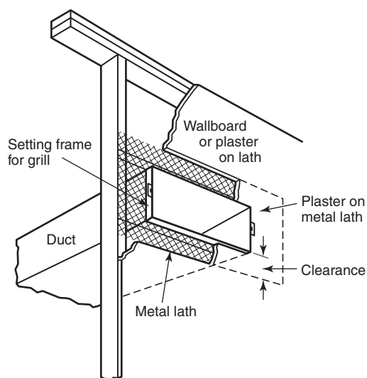
FIGURE 6.1.2.7(a) An Arrangement for Closing Ends of Clearance Space Around a Supply Duct. A similar arrangement can be used where a duct continues through the partition.
