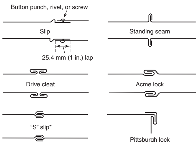
FIGURE 5.3.2.3 Types of Duct Joints.
