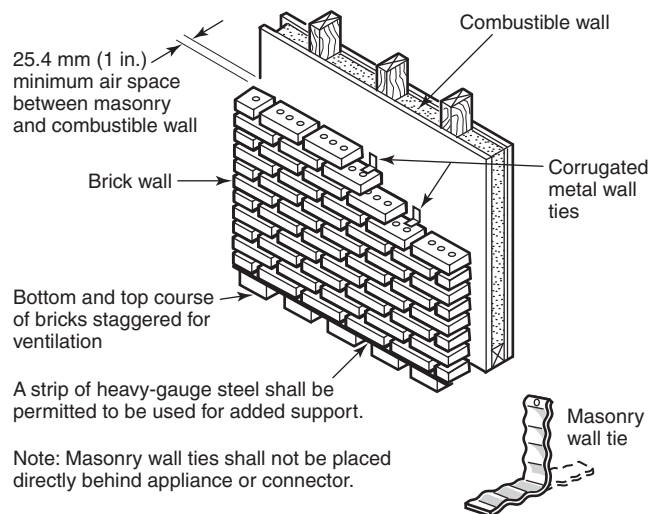
FIGURE 6.1.4.2(c) Masonry Clearance Reduction System.
