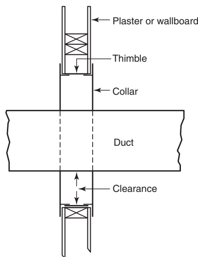
FIGURE 6.1.2.7(b) An Arrangement for Passing Ducts Through Combustible Walls or Partitions as Specified in 5.1.2.5.
