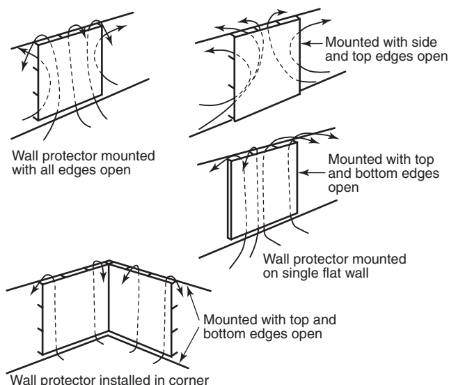
FIGURE 5.1.4.2(a) Sheet Metal or Other Protection to Reduce Required Clearance from Heating Appliance.
