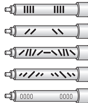
FIGURE D.2.1(e) Leaky Coaxial.
