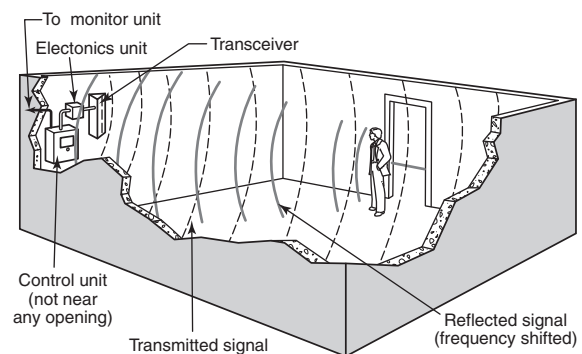
FIGURE D.2.2(g) Microwave.
