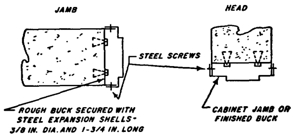
Figure 8. Double type (inverted) frame.
