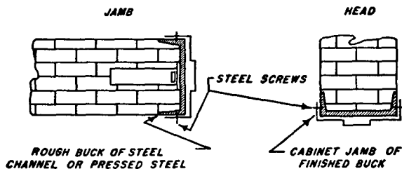
Figure 7. Double type (normal) frame.
