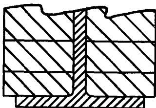
Figure 17. Steel lintel.
