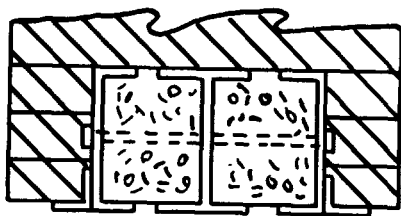
Figure 15. Steel lintel.
