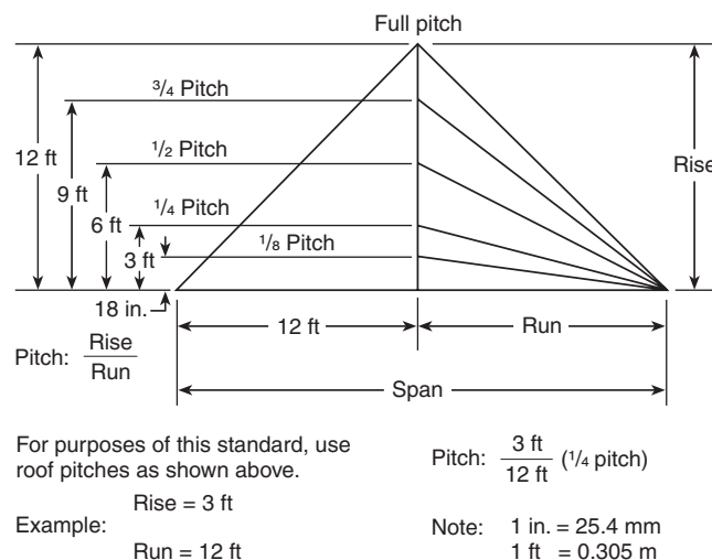
Figure 3-1.2(b) Roof pitch.
