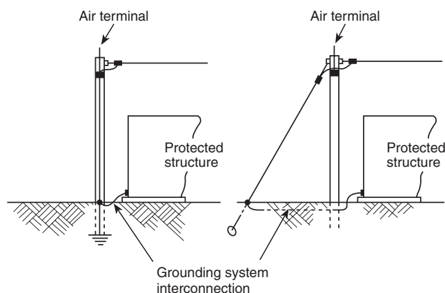
Figure 6-3.3.4 Alternate grounding method for overhead ground-wire protection.
