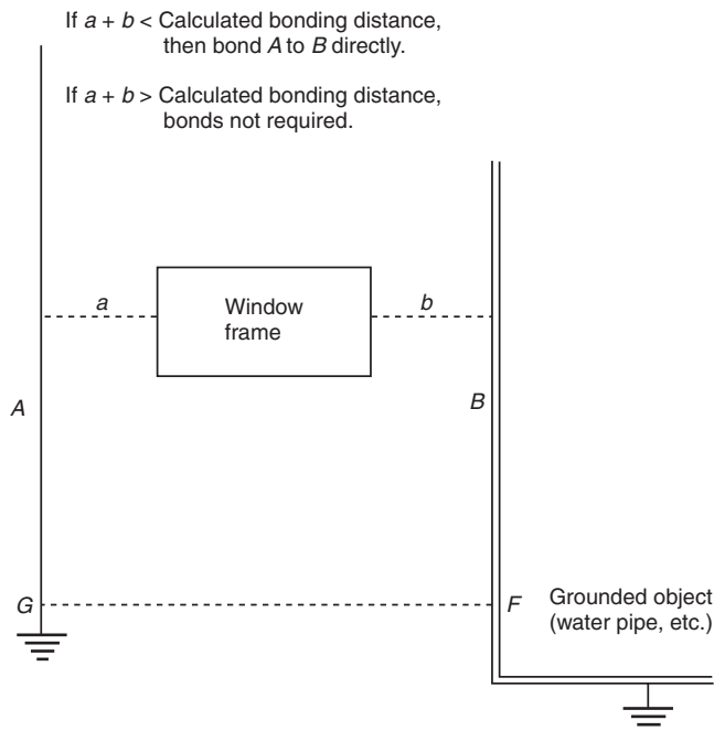
Figure 3-21.3 Effect of isolated (nongrounded) metallic bodies, such as a window frame, in nonconductive media.
