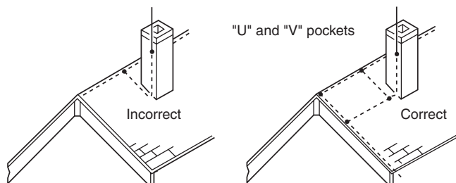
Figure 3-9.4 Pockets.
