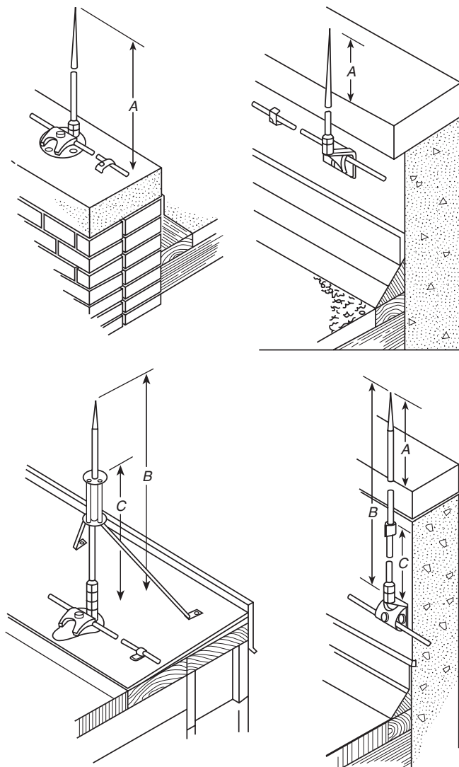
A: 10 in. (254 mm). See 3-6.1. 24 in. (600 mm). See 3-6.2. B: Air terminals over 24 in. (600 mm) high shall be supported. C: Air terminal supports shall be located at a point not less than one-half the height of the air terminal.
