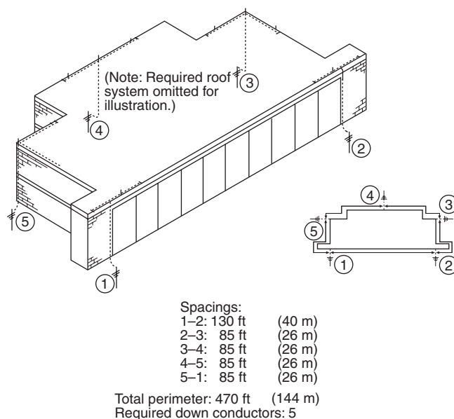
Figure 3-9.10 Quantity of down conductors.
