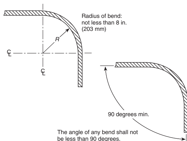
Figure 3-9.5 Conductor bends.
