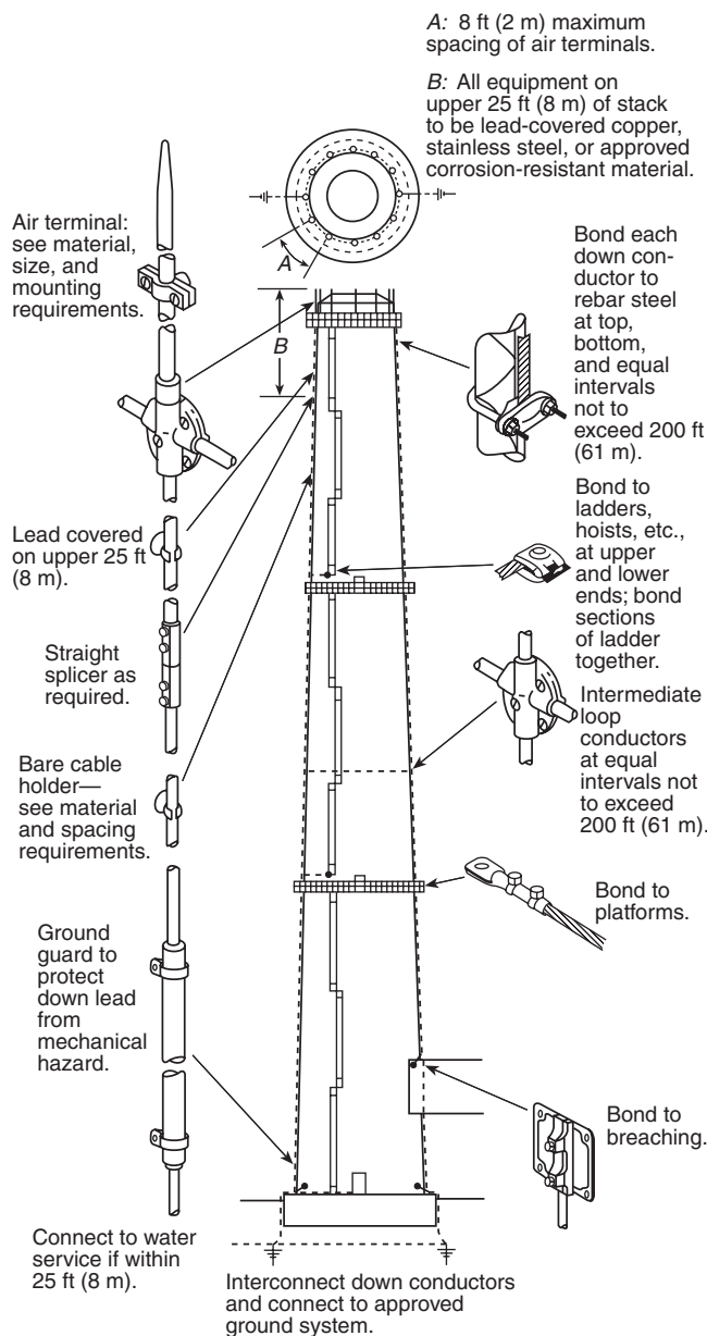
Figure 5-1 Heavy-duty stack.
