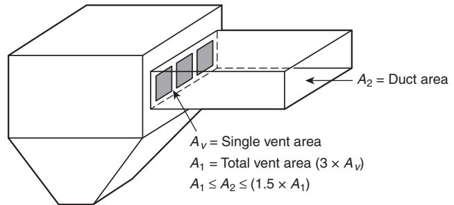
FIGURE 6.8.3 Example Range of Vent Duct Area for Manifolded Vent Duct.
