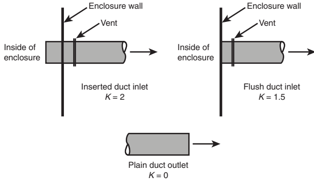
FIGURE A.8.5(a) Loss Coefficients for Inlets and Plain Duct Outlet.
