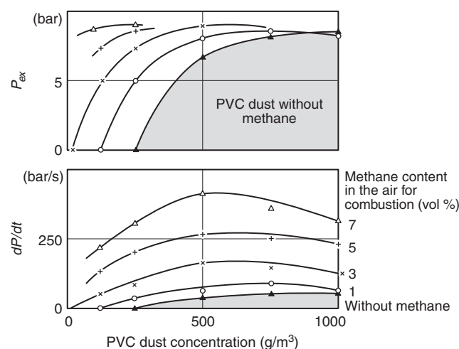
FIGURE B.2.5.2 Deflagration Data for Hybrid Mixtures of Polyvinyl Chloride Dust and Methane Gas in Air [4].
