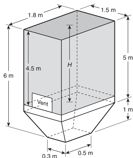
FIGURE A.6.4.3(e) Rectangular Enclosure with a Hopper and a Side Vent Close to the Hopper.
