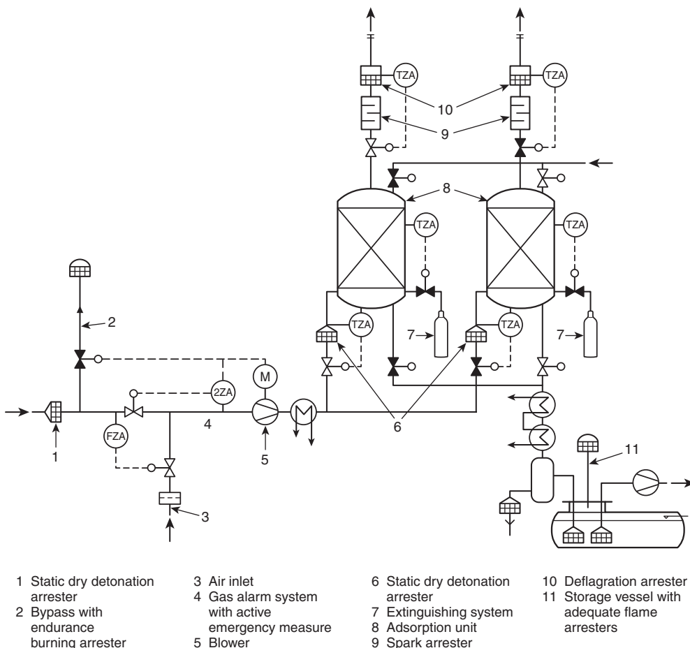
FIGURE 10.4.1 Protection Strategy for a Typical Thermal Regenerated Carbon Adsorption Unit for Solvent Recovery.
