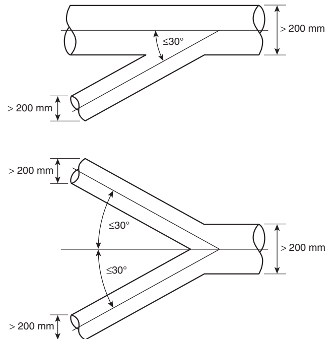
FIGURE 7.5.1.2 Design of Piping for Detonation Containment in Combination with Detonation Arresters. (Source: TRbF 20)
