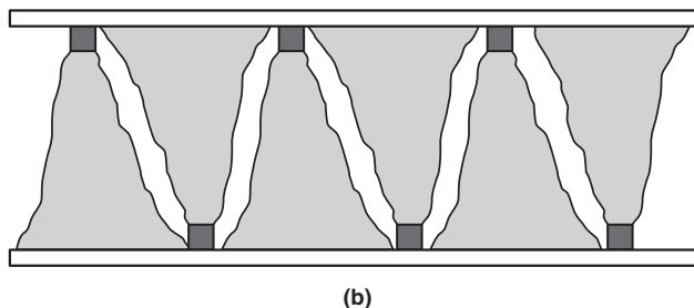
Vertical section on A-A showing the relative positions of spray heads used to promote more uniform distribution and to avoid spray collision, as in (c); overall spray length ca. 1 m
