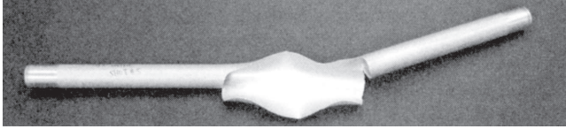
FIGURE 7.7.3.2 Detonation-Induced Rupture in a Flawed Aluminum Tube. (Source: Shepherd, 2009; credit: Linda Hall Library of Science, Engineering & Technology)
