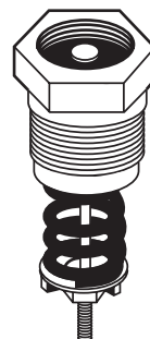
FIGURE A.3.3.69.6.3 Full Internal Pressure Relief Valve.
