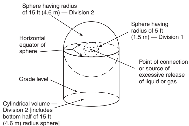
FIGURE A.6.22.2.3 Extent of Electrically Classified Area. (See Table 6.22.2.2.)
