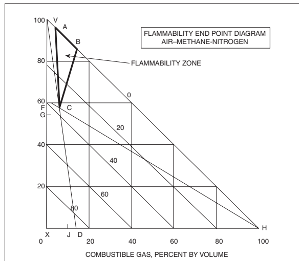
FIGURE 2-2 Flammability end point diagram for the purging of methane with nitrogen at 70° F. The A and B coordinates are 5 and 14 percent methane, and 0-percent nitrogen, respectively. The C coordinate is a mixture of approximately 6 percent methane, 36 percent nitrogen and 58 percent air. The triangle formed by the coordinates of A, B and C represent the flammability zone at 70 degrees F. Note: the flammability zone area will increase as the temperature increases.
