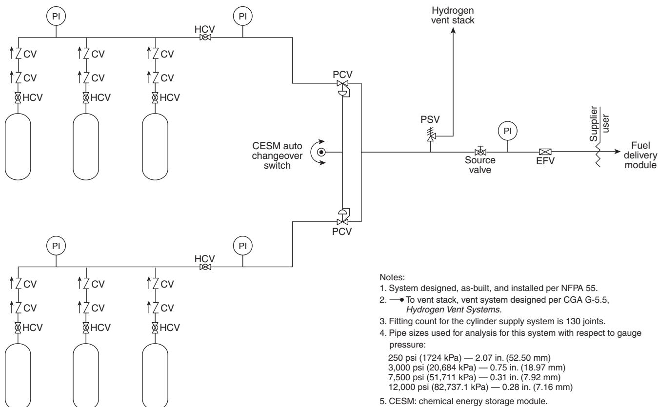
FIGURE A.3.3.95.9.1(e) Typical Chemical Energy Storage Module (CESM).
