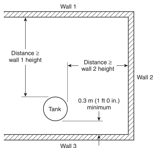
FIGURE A.8.12.2.7.2.1 Bulk Cryogenic System Located in a Courtyard.
