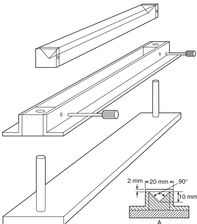
FIGURE A.4.2.5 Fixture for Preparation of Sample for Burning Rate Test.
