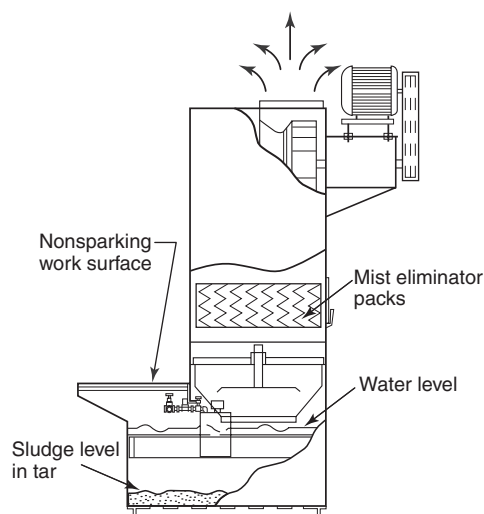
FIGURE A.11.7.3.3.7 Typical Liquid Precipitation Collector for Fixed Dust-Producing Equipment.
