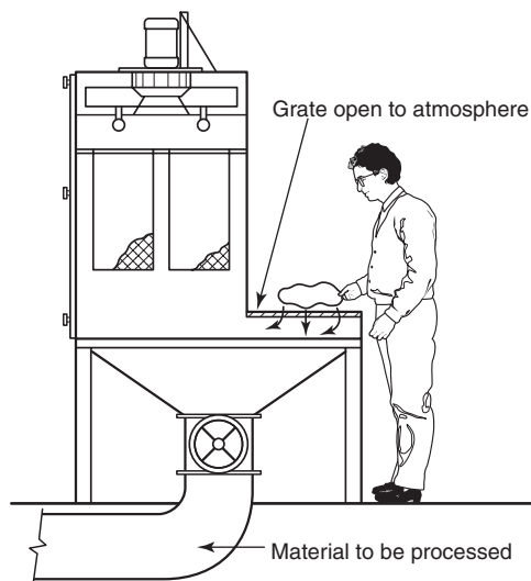
FIGURE A.8.6.4.1(a) Example of Unacceptable Manual Bag Dump Station in Which Operator Is Exposed to Potential Fire or Explosion.
