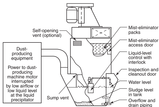
FIGURE A.8.7.3.21.3.3(a) Typical Liquid Precipitation Collector for Fixed Dust-Producing Equipment.
