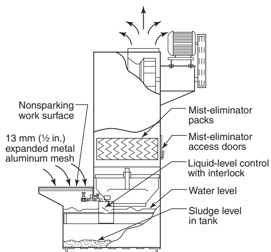
FIGURE A.8.7.3.21.3.3(b) Typical Liquid Precipitation Collector for Portable Dust-Producing Equipment.
