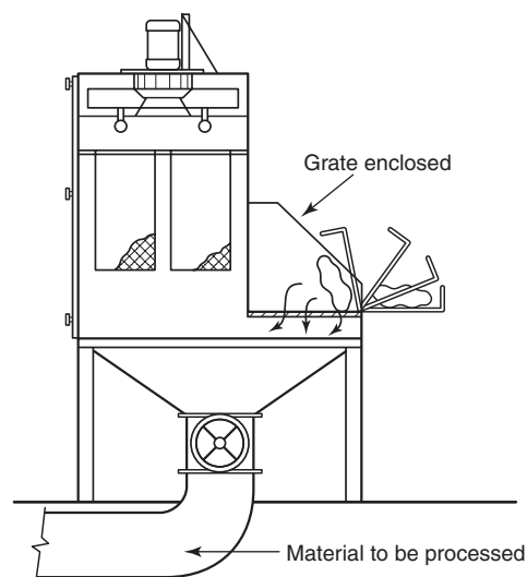
FIGURE A.8.6.4.1(b) Example of Acceptable Station in Which Bag Dump Operation Is Automatic.
