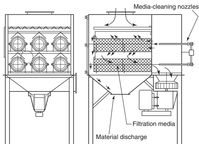
FIGURE A.8.7.3.5 Example of a Fixed Media-Type Dust Collector.
