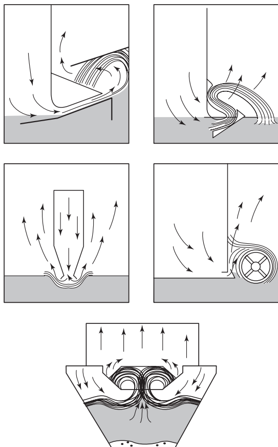
FIGURE A.8.7.3.21.3.3(c) Five Methods of Precipitating Dust in Precipitators.
