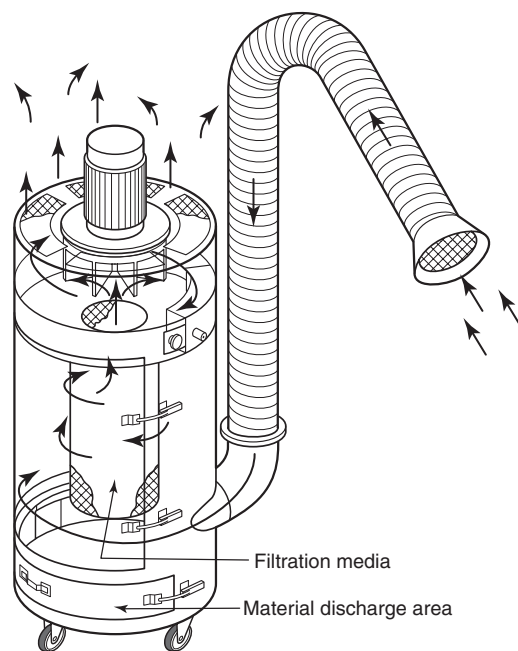
FIGURE A.8.7.3.5.1 Example of a Portable Media-Type Dust Collector.
