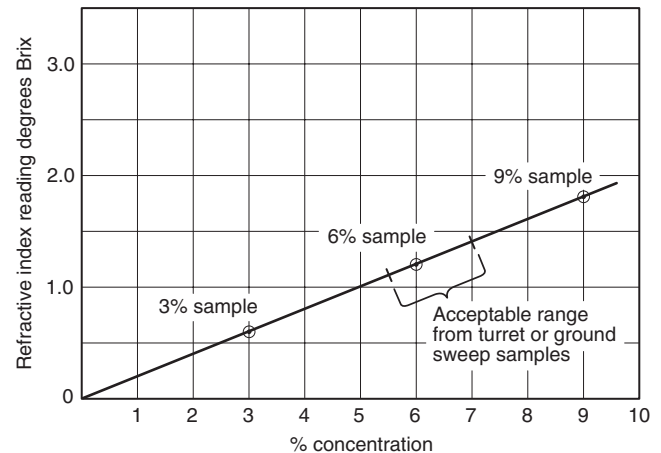
Figure A-4-3.2(a) Typical graph using AFFF (6%).
