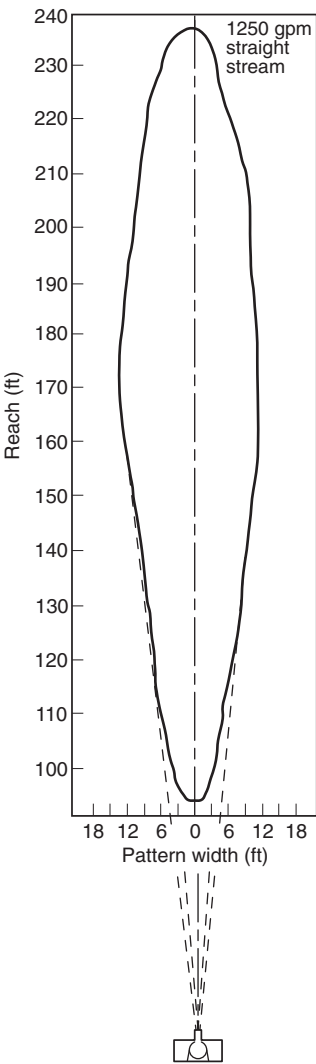
Figure A-4-5.2 Typical foam discharge pattern.
