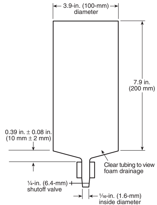
Figure 4-3.3.1.2 1600-mL foam sample container.
