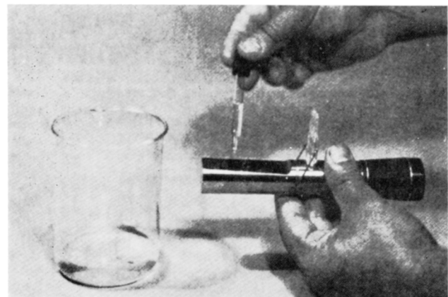
Figure A-4-2.2(a) Measuring the index of refraction by placing a few drops of the solution to be tested on the prism of a refractometer and closing the cover plate. This is a typical refractometer suitable for this purpose.
