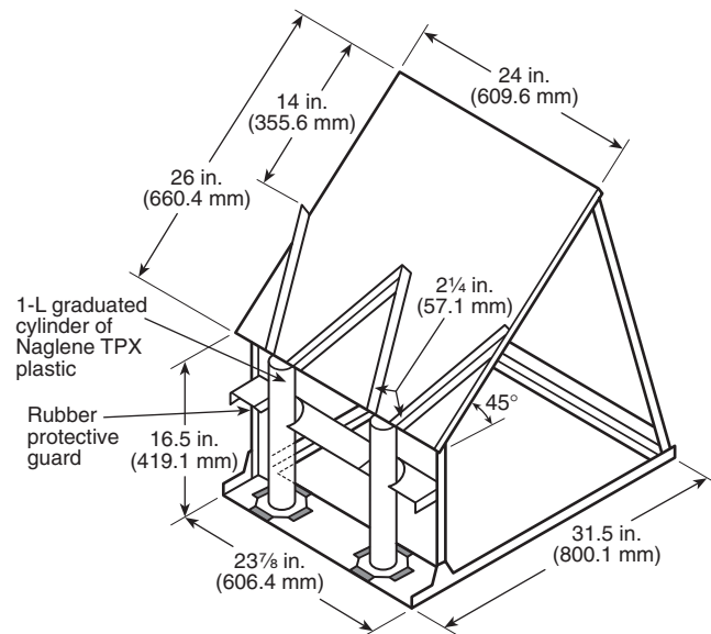
Figure 4-3.2.1.1 Aqueous film forming foam sample collector.
