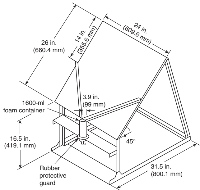
Figure 4-3.3.1.1 Foam sample collector.
