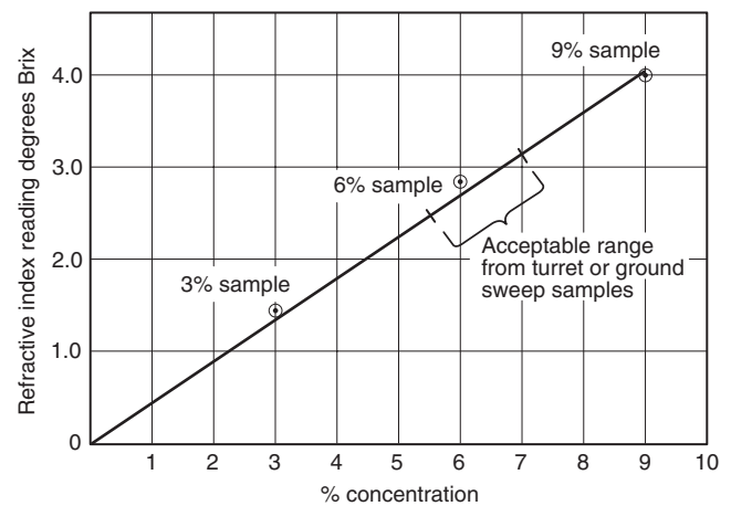
Figure A-4-3.2(b) Typical graph using FFFP (6%).
