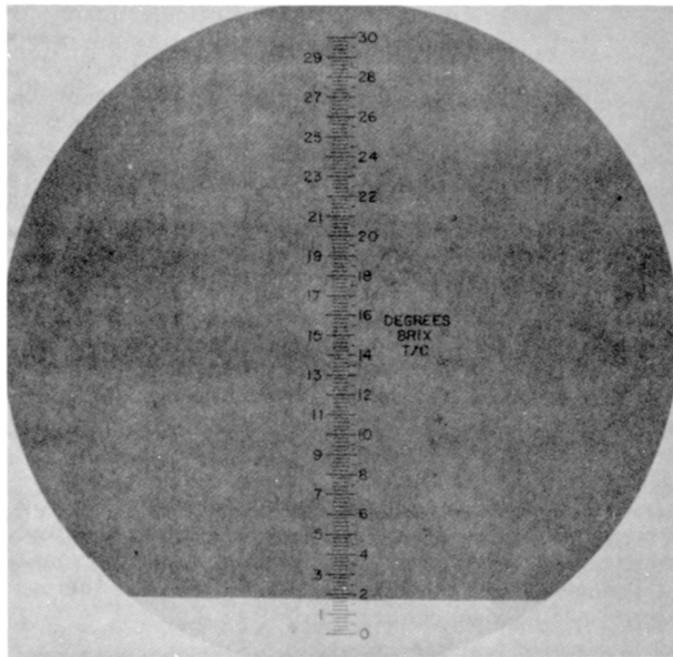
Figure A-4-2.2(c) Illustrating the field of view by looking into the refractometer shown in Figures A-4-2.2(a) and A-4-2.2(b) containing a 6 percent AFFF solution. The dark intersects the scale at 1.7, and this value is recorded as the reading for a 6 percent concentration.
