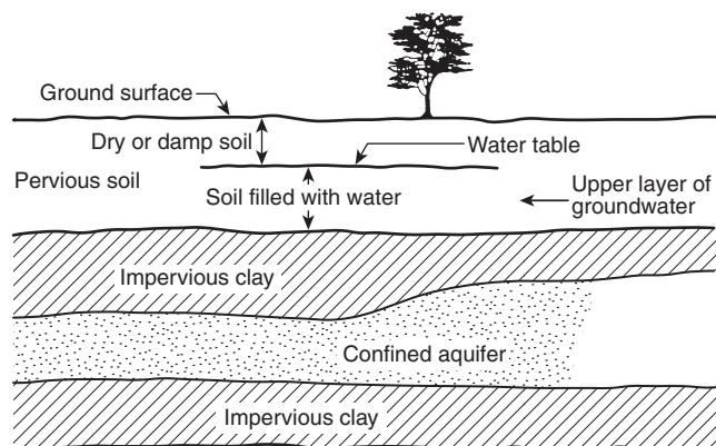
FIGURE C.3 Layering of Groundwater Between and Above Impervious Strata.
