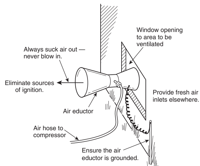
FIGURE 5.4.7.1 Exhaust Ventilation.
