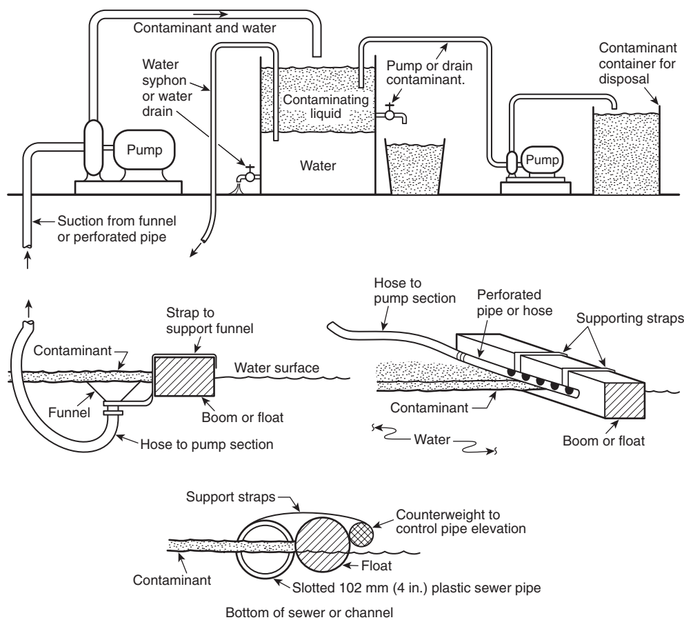
FIGURE 9.5.4(a) Typical Skimming Installation.
