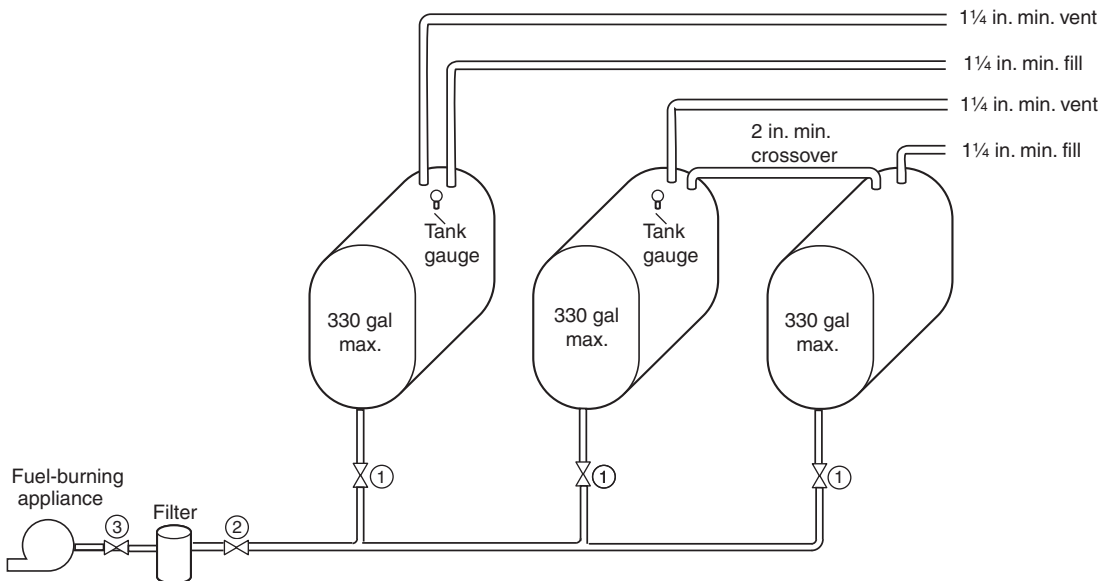
FIGURE 8.9.1 Cross-Connection of Two Fuel Tanks of Not More Than 660 gal (2500 L) Aggregate Capacity.
