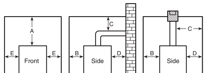
FIGURE 10.6.1 Clearances to Combustible Materials.
