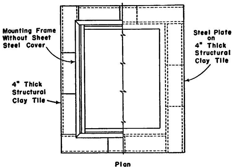
Figure 4. Installation of Downflow Furnace on Combustible Floor.
