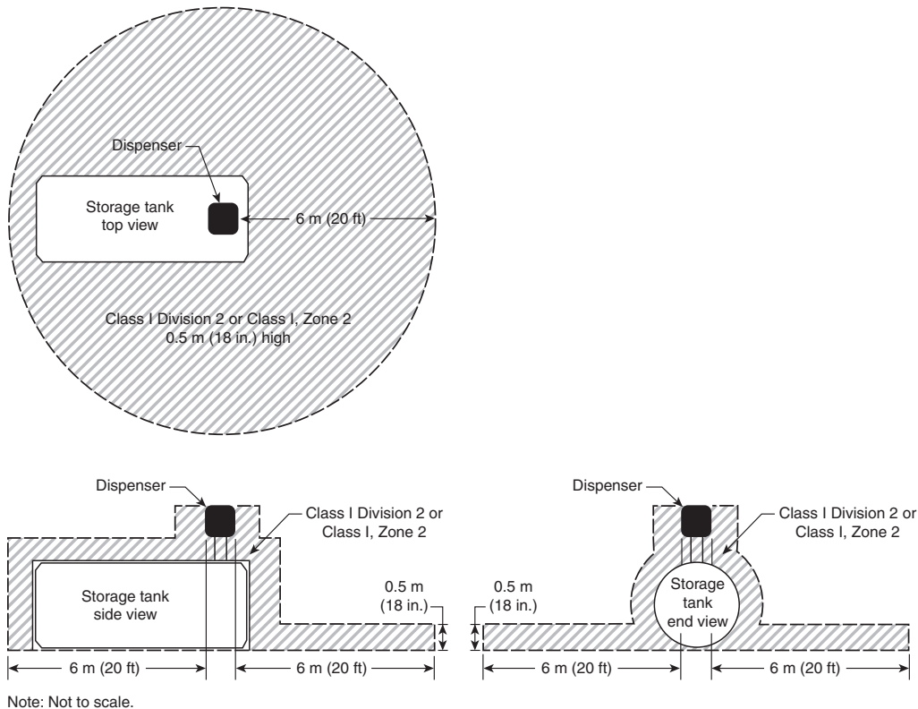
FIGURE 8.3.3(b) Classified Areas Adjacent to Dispenser Mounted on Aboveground Storage Tank.
