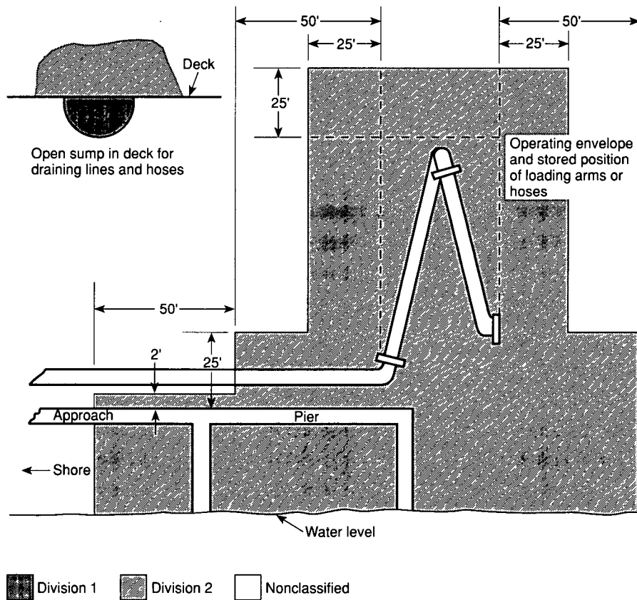
Figure 5-3.5.6 Marine terminal handling flammable liquids.
