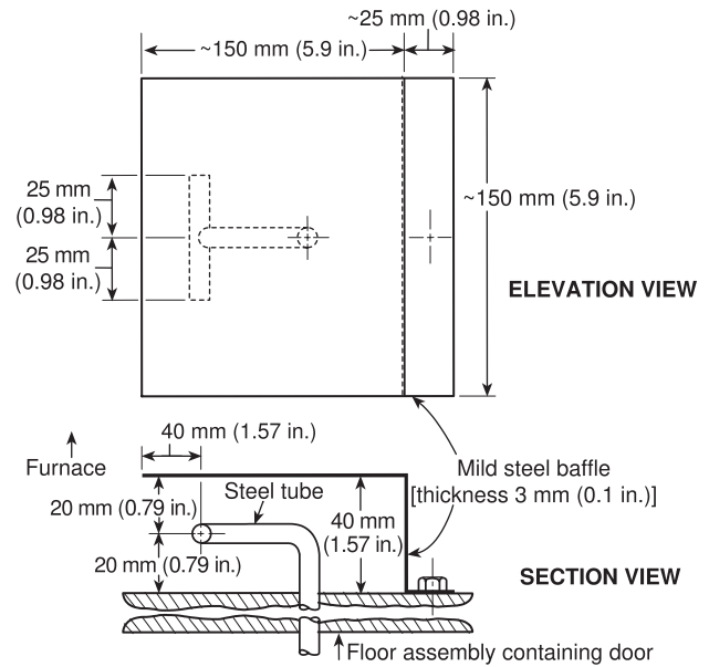
FIGURE 4.4.1(a) Static Pressure-Measuring Device Dimensions.
