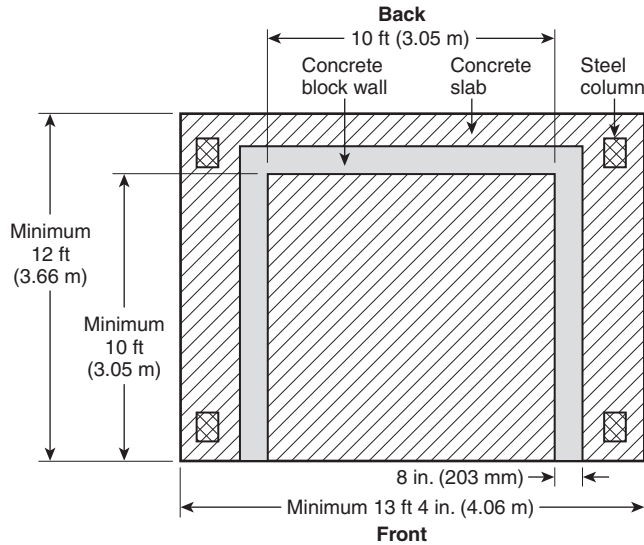
FIGURE A.4.4.3(a) Plan View of Test Apparatus — Both Stories (not to scale).
