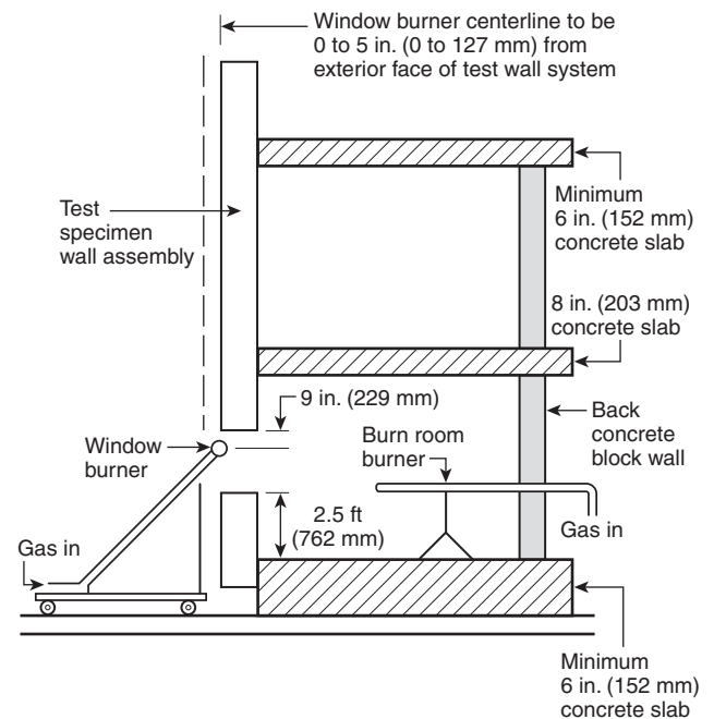
FIGURE A.4.6.3.6 Section View of Burner Placements for First-Story Test Room (not to scale).
