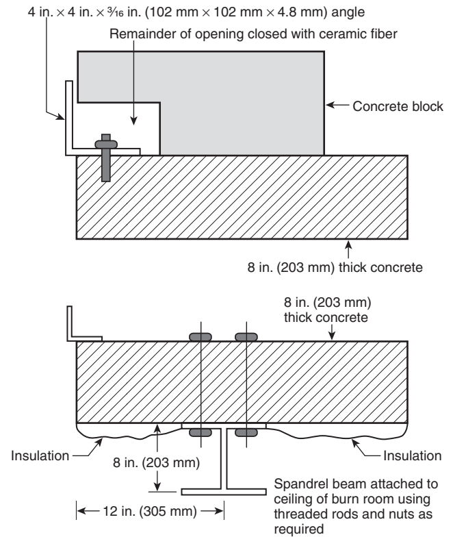
FIGURE A.4.4.3(c) Details A and B. Also see Figure A.4.4.3(b) (not to scale).
