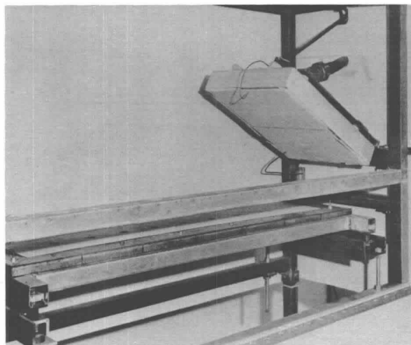
Figure 2-1B Flooring Radiant Panel Test Showing Carpet Specimen and Gas-Fueled Panel.
