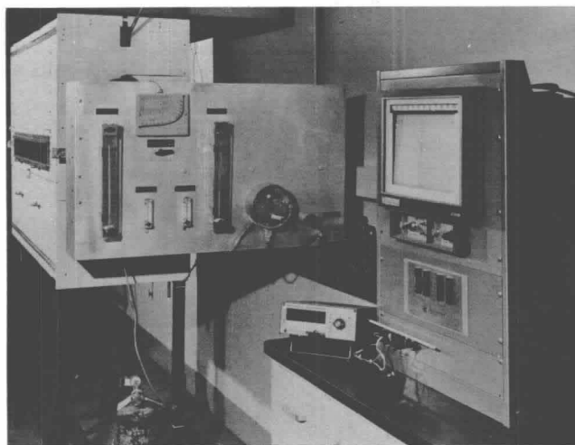
Figure 2-1A Flooring Radiant Panel Tester Apparatus.
