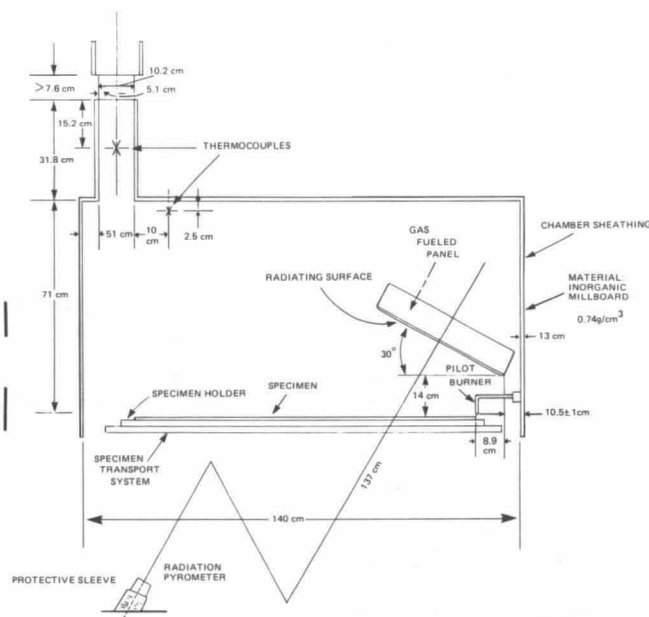
Figure 2-3A Flooring Radiant Panel Tester Schematic — Side Elevation.
