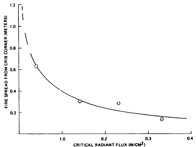
Figure E-4 Room Burn Tests: Fire Spread from Crib Along Floor Covering; 6.4 kg (14 lb) Wood Crib.
