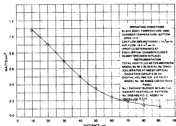
Figure 1-3.1 Standard Radiant Heat Energy Flux Profile.
