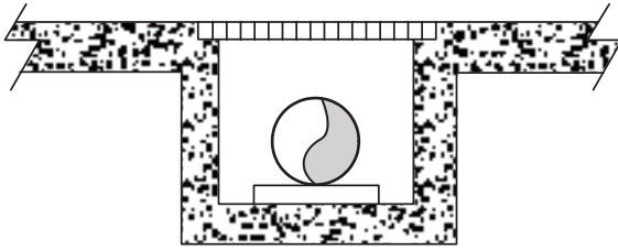
N FIGURE A.10.4.3.2.1 Private Service Main in a Covered Trench.
