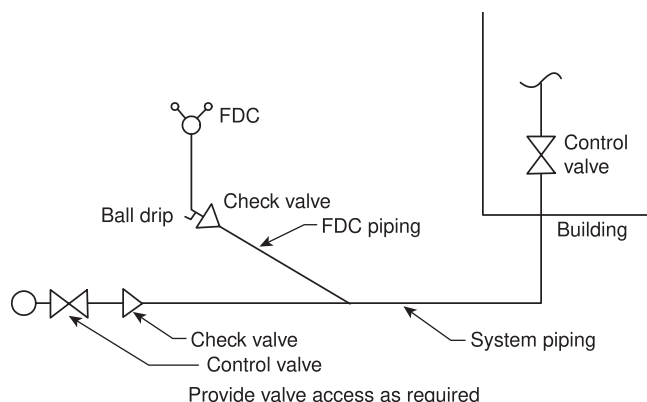
FIGURE A.5.9.3.2.1(a) Fire Department Connection Connected to Underground Piping (Sample 1). [13:Figure A.16.10.4.4(a)]
