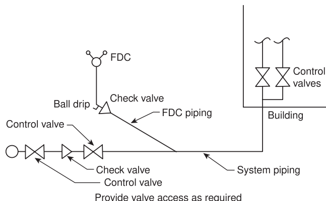
FIGURE A.5.9.3.2.1(b) Fire Department Connection Connected to Underground Piping (Sample 2). [13:Figure A.16.10.4.4(b)]
