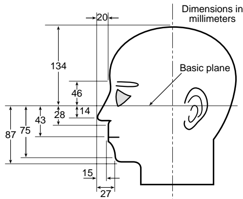
FIGURE 6-20.4.1.1 Alderson headform.
