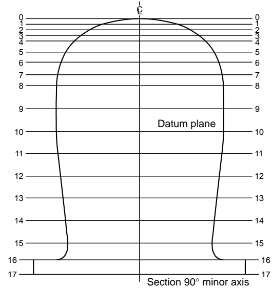
FIGURE 6-18.4.1(c) Size 7 headform, front.
