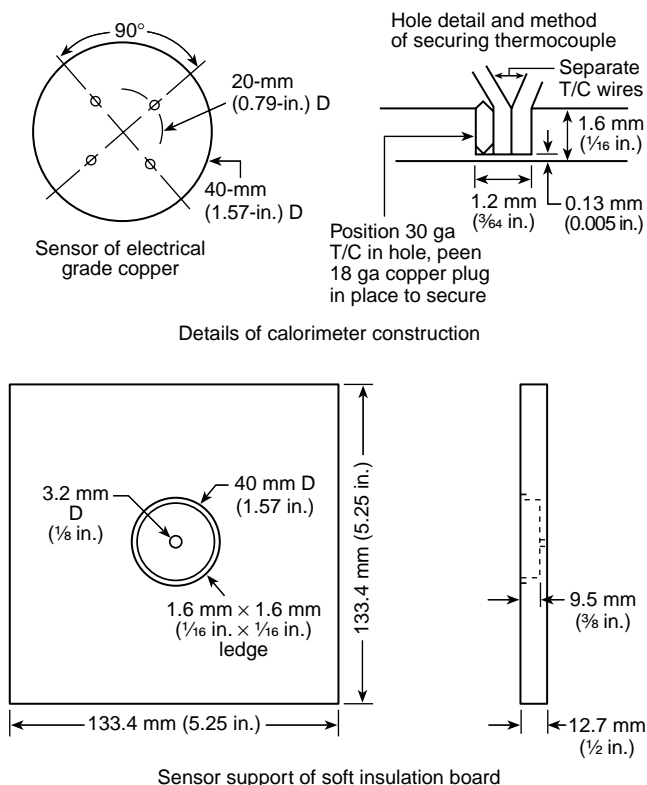
FIGURE 6-10.4.4 Sensor assembly.
