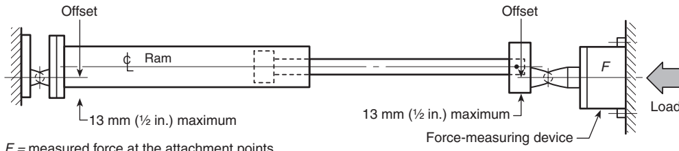
FIGURE 8.12.1 Fixture for Ram Bend Test.
