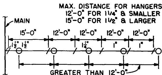
Fig. 3-14.5. Distance Between Hangers.
