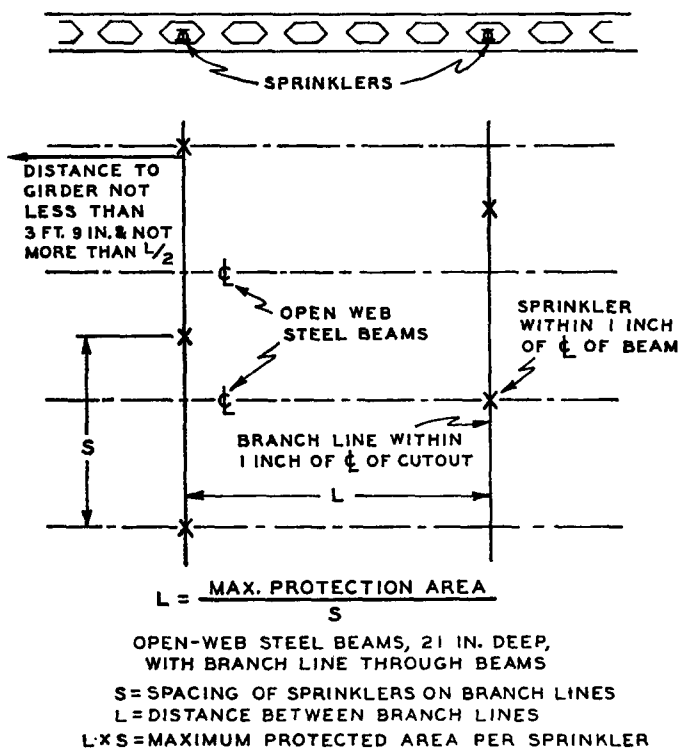
Fig. 4-2.4.4. Location of Branch Lines and Sprinklers.
