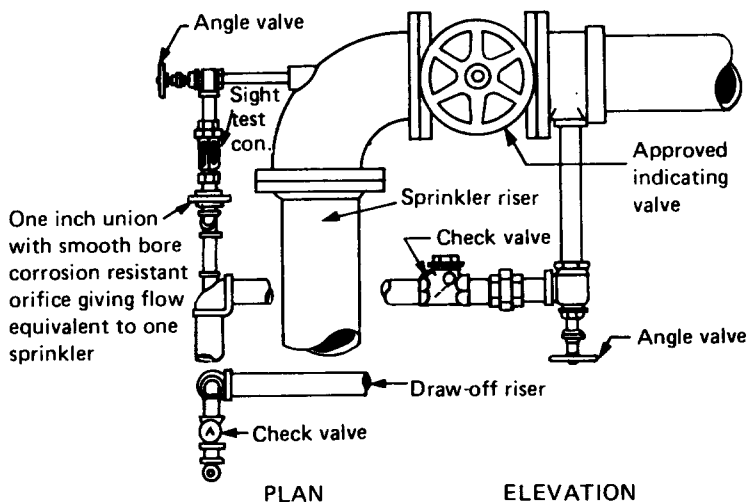
Fig. A-3-8.1.1 (b) One-Inch System Test Pipes on Wet-Pipe Systems.
