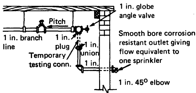
Fig. A-3-8.2 One-inch System Test Pipes on Dry-Pipe Systems.
