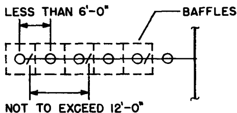
Fig. 3-14.6.4. Distance Between Hangers. (See 3-14.6.4 and 4-4.19.)
