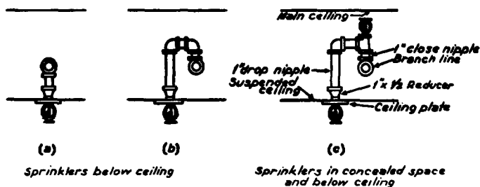
Fig. 3-7.4. Pendent Sprinklers at Suspended Ceiling.
