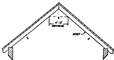
Fig. 7208(a)(4). Desirable Horizontal Clearance for Sprinklers at Peak of Pitched Roof.
