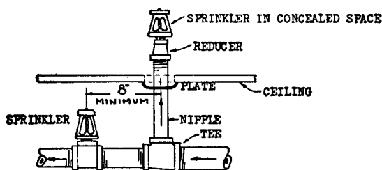
Fig. 4212-2. Sprinkler on Riser Nipple from Branch Line in Lower Fire Area.
