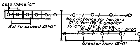
Fig 533(a)2. Distance Between Hangers.
