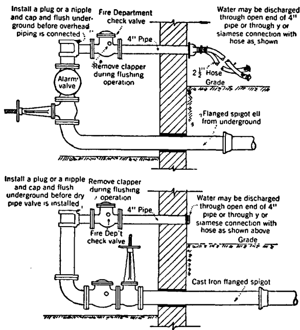
Fig. 112. Methods of Flushing Water Supply Connections.
