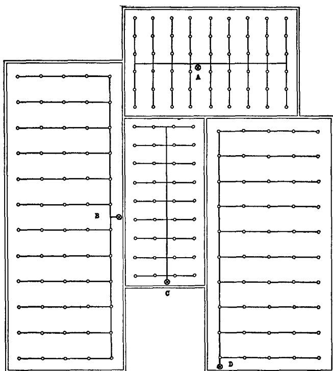
Fig. 4301. Location of Risers.
