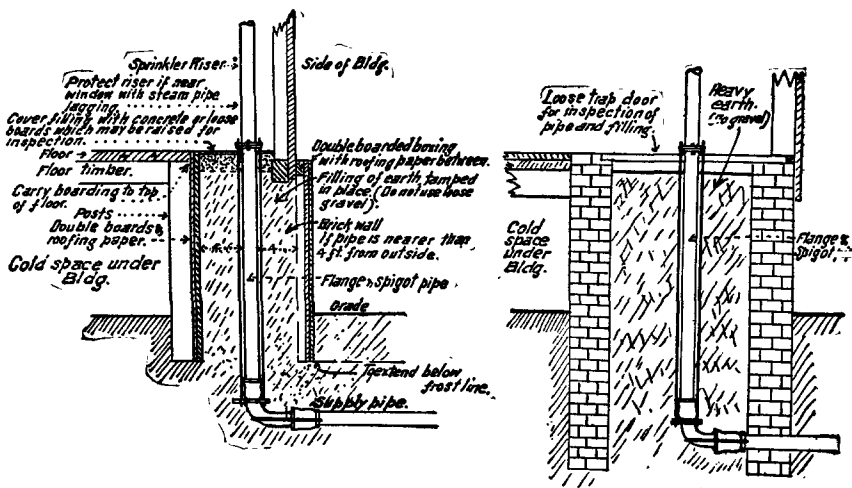
Fig. 4610. Protection of Sprinkler Risers Against Freezing.
