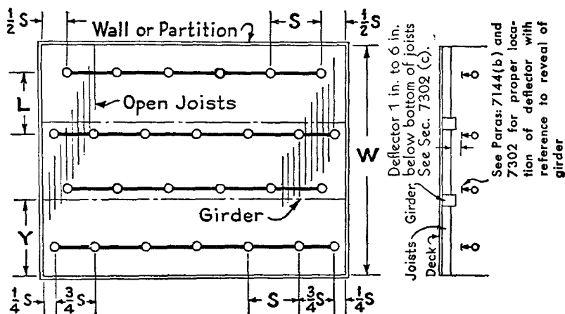
Sprinklers on Alternate Lines Staggered
