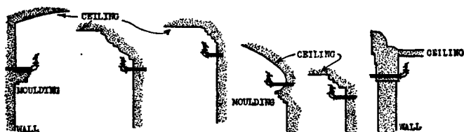
Fig. 7403. Suggested Arrangements for Sidewall Sprinklers — placed to receive early heat waves and provide effective distribution.
