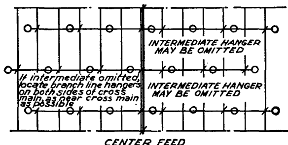
Fig. 533(b)3. Hangers on Cross Main — Center Feed System.
