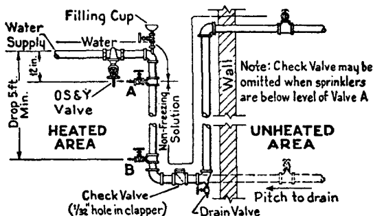
Fig. 903. Arrangement of Supply Piping and Valves.
