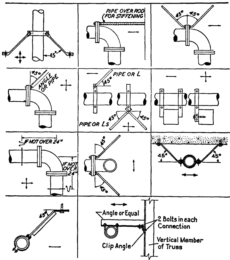
Fig. 4828. Acceptable Types of Sway Bracing.
