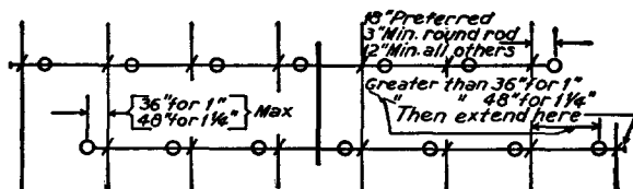
Fig. 533(a)1. Distance from Sprinkler to Hanger.
