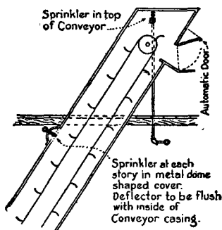
Fig. 7222(a). Sprinklers in Conveyor Enclosure.
