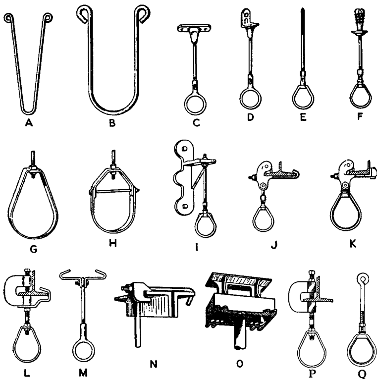
Fig. 531. Common Types of Acceptable Hangers.
