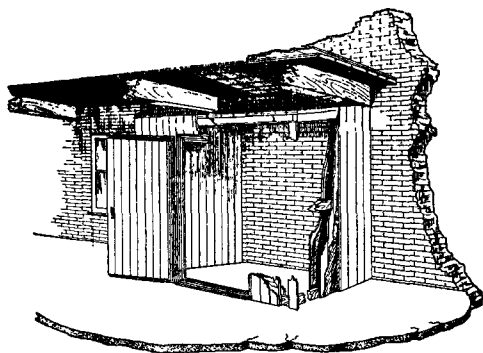
SECTIONAL VIEW
