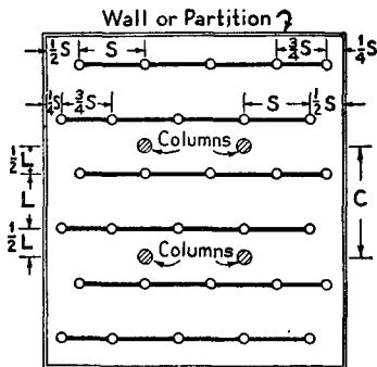
Sprinklers on Alternate Lines Staggered When either L or S is 12 ft. 1 in. to 15 ft.
