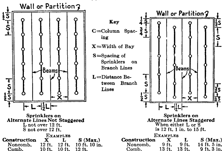
Fig. 7115(c). Layout of Sprinklers Under Smooth Ceiling Construction — Ordinary Hazard.
