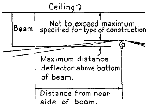
Fig. 7302. Position of Deflector When Located Above Bottom of Beam.
