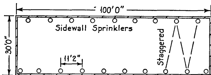
Fig. 7402. Spacing of Sidewall Sprinklers under Smooth Ceilings, with Light Hazard Occupancy.
