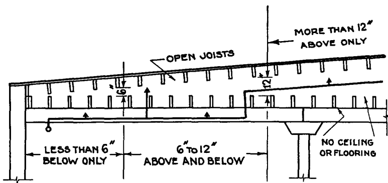
Fig. 7144(c). Arrangement of Sprinklers under Two Sets of Open Joists — no sheathing on lower joists.
