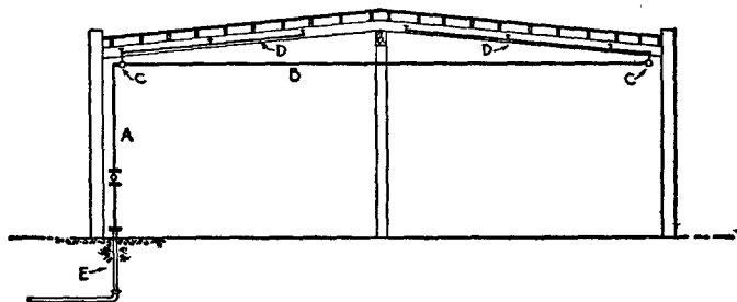
Fig. 4100. Building Elevation Showing Parts of Sprinkler Piping System. A — Riser; B — Feed Main; C — Cross Main; D — Branch Line; E — Underground Supply.
