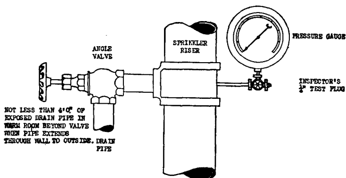
Fig. 4420. Drain Connection for Sprinkler Riser.
