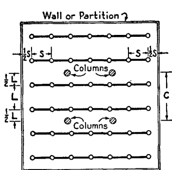
Sprinklers on Alternate Lines Not Staggered L not over 12 ft. S not over 12 ft.
