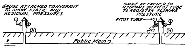
Fig. 315. Method of Conducting Flow Tests.
