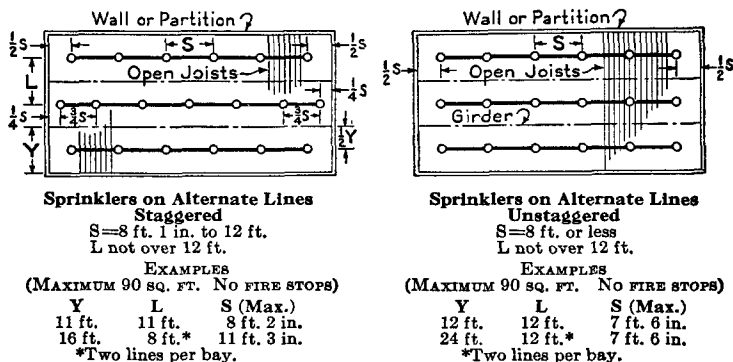
Fig. 7142(a). Layout of Sprinklers Under Open Joist Construction — Light and Ordinary Hazard Occupancy. [For Key to symbols see Fig. 7144(b).]
