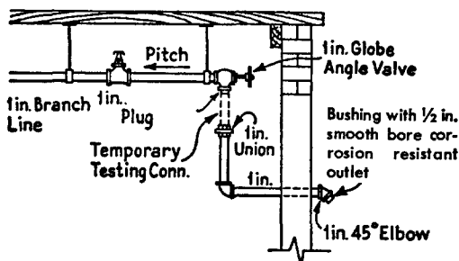
Fig. 4503. One-inch System Test Pipes on Dry-Pipe Systems.
