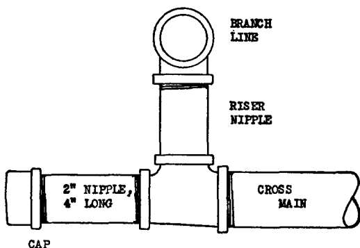
Fig. 4304. Flushing Connection.
