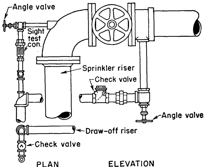
Fig. 4501. One-Inch System Test Pipes on Wet-Pipe Systems. Connect to top of main riser or to sprinkler pipe in the highest part of system.
