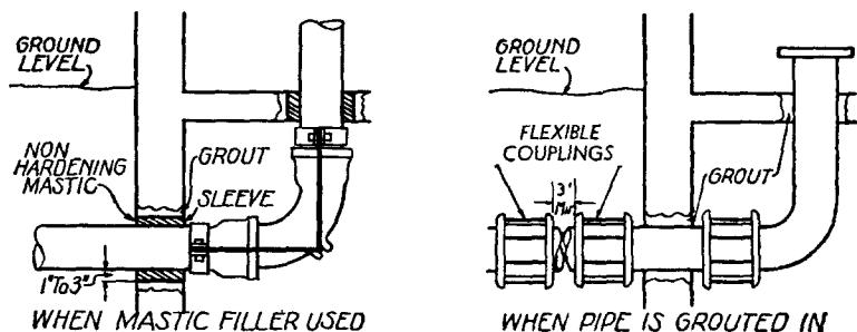
Fig. 4800. Arrangement of Supply Pipe Entering Building.
