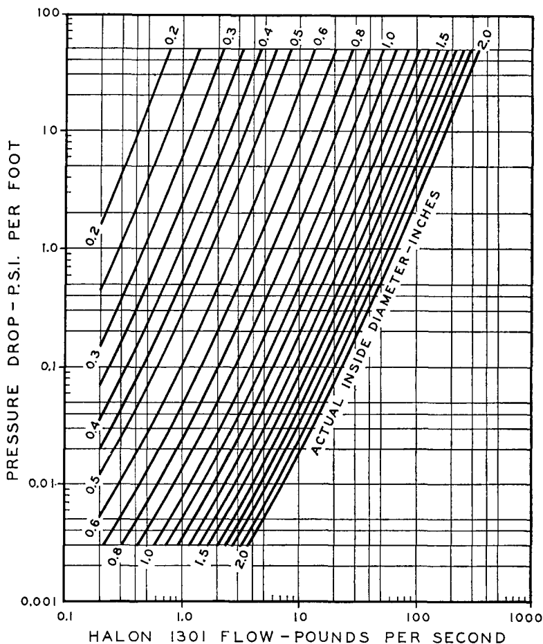
Fig. 2. Pressure drop vs. flow in copper tubing.
