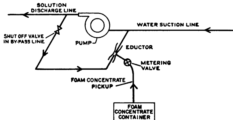
Figure A-4-1 Around-the-Pump Proportioning System Typical Arrangement.
