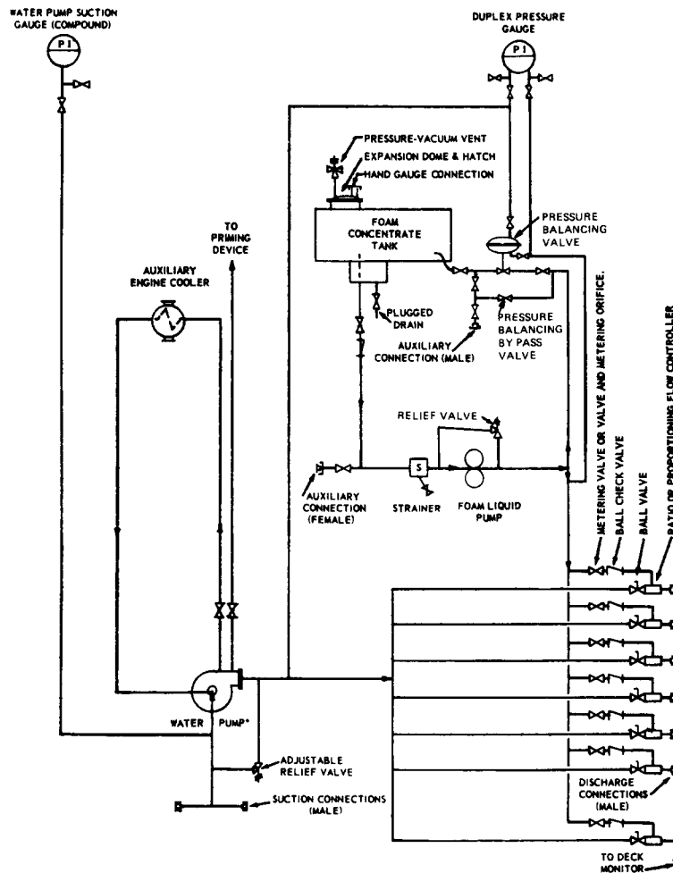
Figure A-3-1 Typical Balanced Pressure Proportioning System.
