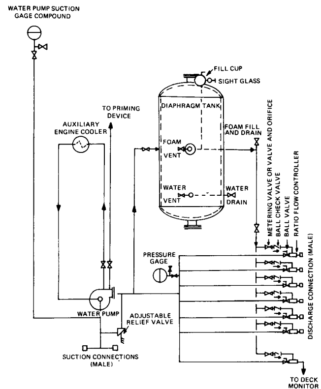
Figure A-6-1 Pressure Proportioning Diaphragm Tank Method.
