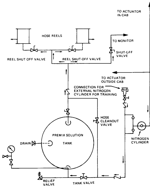
Figure A-5-1 Typical Truck Mounted AFFF Premixed Solution System.
