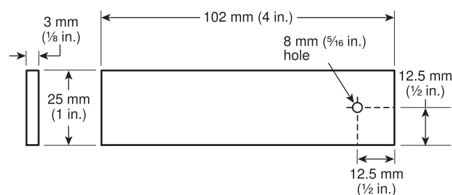
FIGURE 5.5.1.5 Test Coupon.
