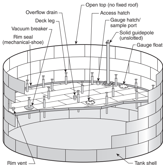
N FIGURE A.3.3.31.2(a) External Floating Roof System. (Source: Rob Ferry, P.E., Trinity Consultants, Inc.)
