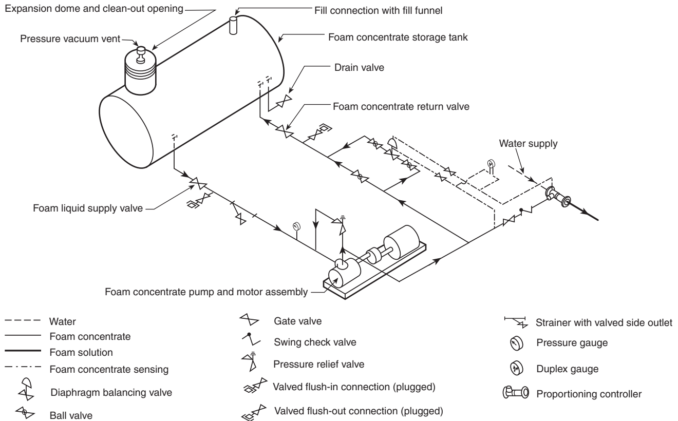
N FIGURE A.4.5.2.2(d) Balanced-Pressure Proportioners (with Concentrate Pump).
