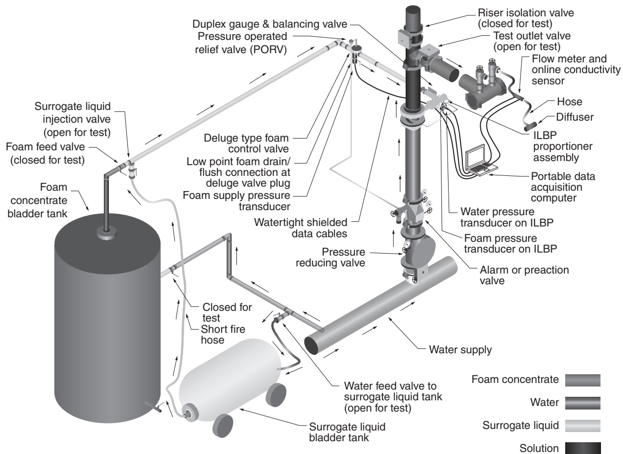
N FIGURE D.5.2.2(e) Bladder Tank In-Line Balanced Pressure Proportioning System Setup for Surrogate Liquid Type Test.
