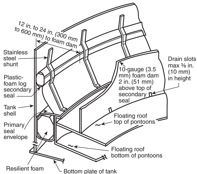
Δ FIGURE 5.3(d) Double Seal System for Floating Roofs Using Plastic-Foam Log (Secondary Seal).
