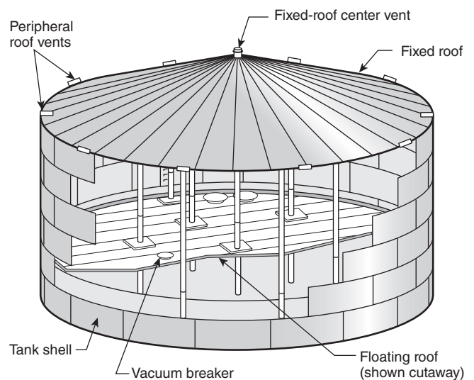
N FIGURE A.3.3.31.3 Internal Floating Roof System With Fixed Cone or Dome Roof Covering. (Source: Rob Ferry, P.E., Trinity Consultants, Inc.)
