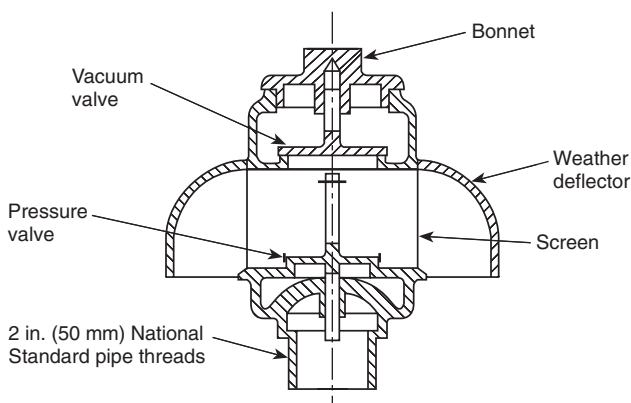
N FIGURE A.13.3.2.5.5.3(2) Pressure Vacuum Vent. [25:Figure A.3.3.34]
