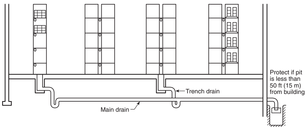
N FIGURE A.6.5.2.6.1(a) General Scheme for Warehouse Spill Control of Liquids. [30:Figure A.16.8.2(a)]
