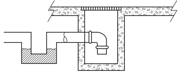
N FIGURE A.6.5.2.6.1(e) Details of Liquid-Seal Trap. [30:Figure A.16.8.2(e)]
