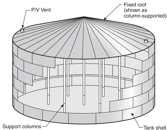
N FIGURE A.3.3.31.1 Cone/Dome Roof System. (Source: Rob Ferry, P.E., Trinity Consultants, Inc.)
