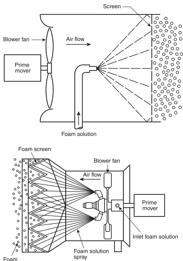
FIGURE A.7.4(c) Blower-Type Foam Generators.
