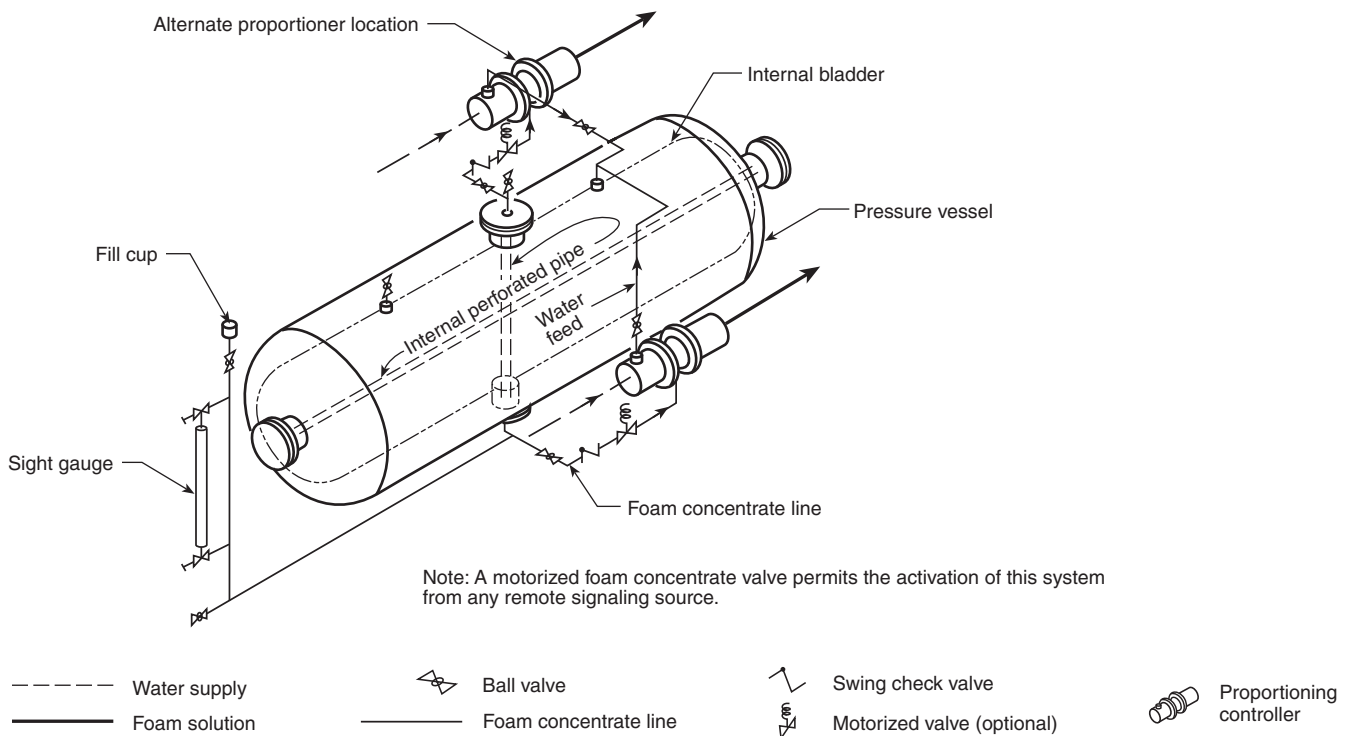
N FIGURE A.4.5.2.2(e) Balanced-Pressure Proportioning (Bladder System).
