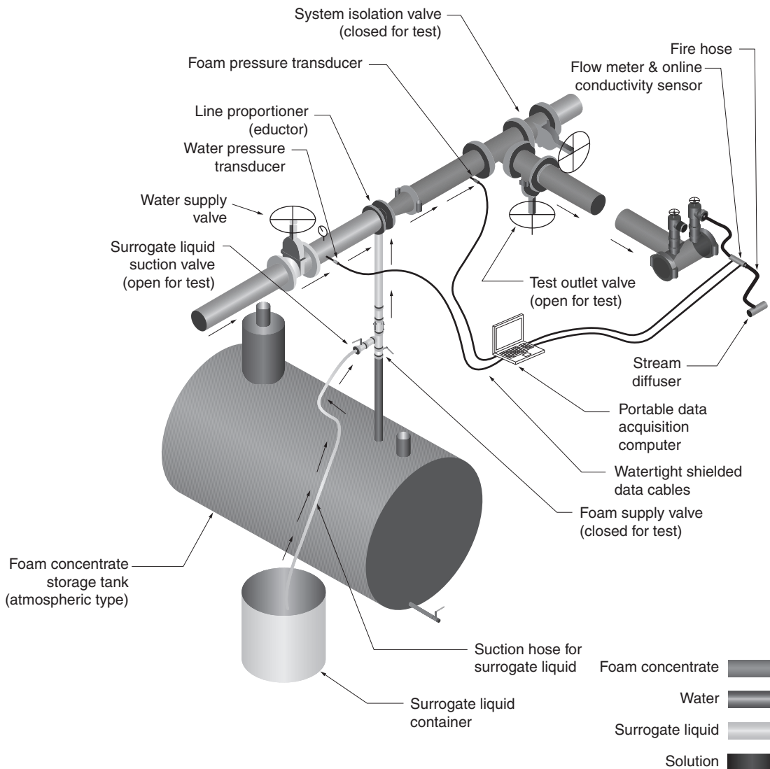
N FIGURE D.5.2.2(f) Atmospheric Tank Eductor Proportioning System Setup for Surrogate Liquid Type Test.
