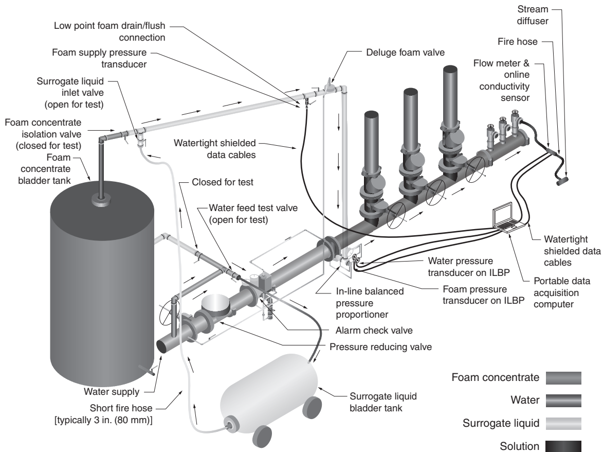
N FIGURE D.5.2.2(d) Bladder Tank Low Flow Proportioning System Setup for Surrogate Liquid Type Test.
