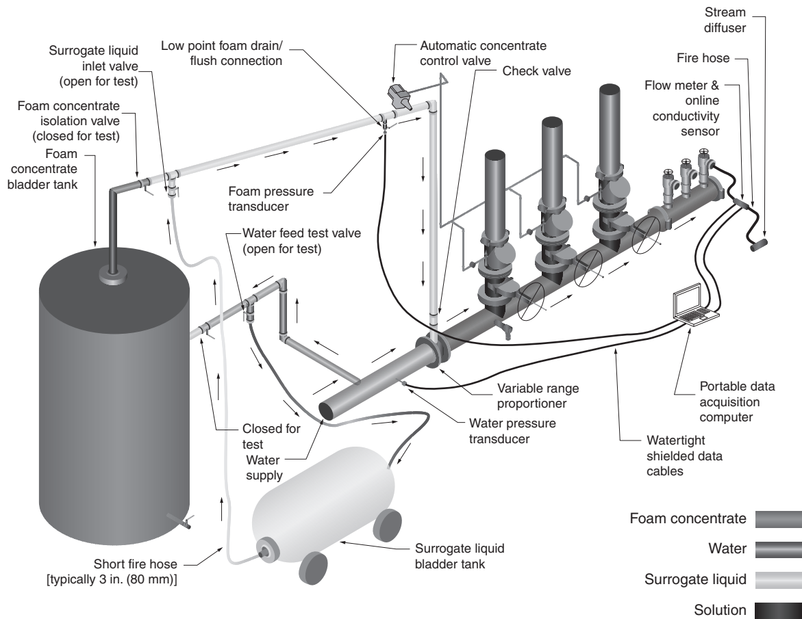
N FIGURE D.5.2.2(c) Bladder Tank Variable Range Proportioning System Setup for Surrogate Liquid Type Test.
