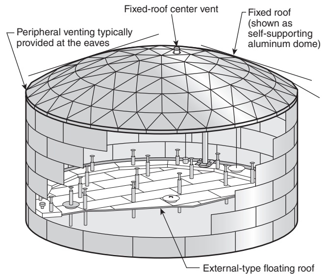
N FIGURE A.3.3.31.2(b) External Floating Roof System with Geodesic Dome (Considered External Floating). (Source: Rob Ferry, P.E., Trinity Consultants, Inc.)
