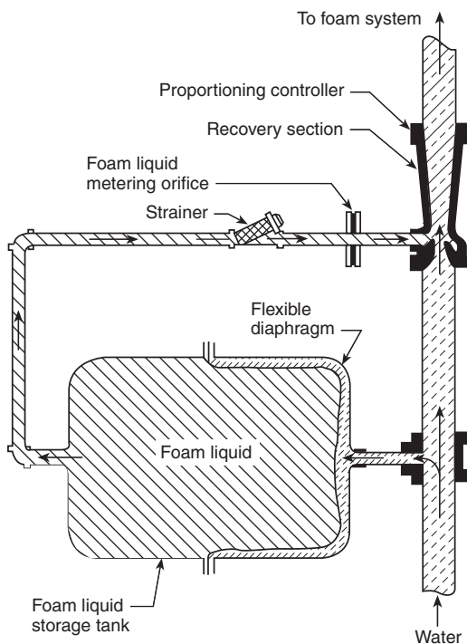
N FIGURE A.4.5.2.2(h) Pressure Proportioning Tank with Diaphragm.
