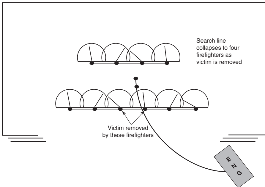
N FIGURE A.7.6.2.3(d) Search Line Shrinking and Continuing Forward After Victims Are Found and Removed.
