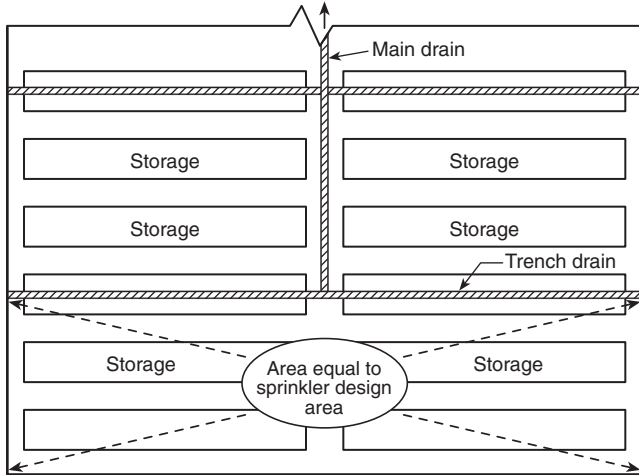
N FIGURE A.6.5.2.6.1(b) Plan View of Warehouse Spill Control of Liquids. [30:Figure A.16.8.2(b)]
