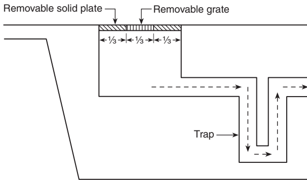
N FIGURE A.6.5.2.6.1(c) Details of Drainage Trench Design. [30:Figure A.16.8.2(c)]
