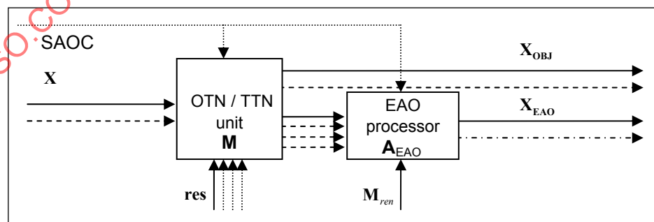
Figure 16 – Architecture of the residual processor
