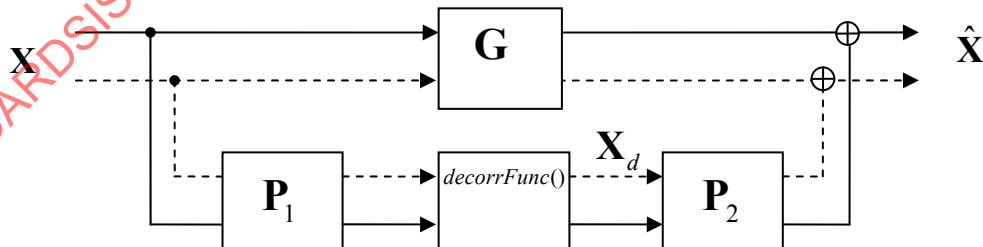
Figure 15 – Basic structure for the SAOC transcoding/decoding modes
