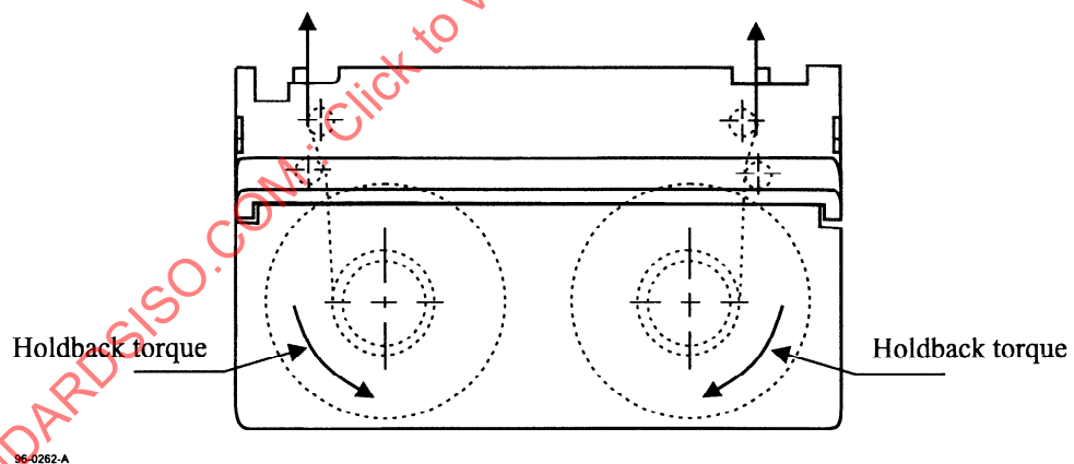
Figure 17 - Tape path to measure the extraction force of Type S cassette
