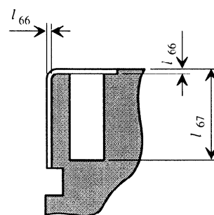
Section H - H
