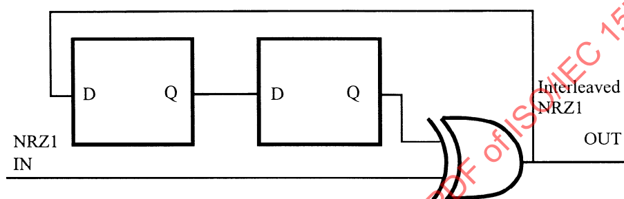
Figure 51 - Precode circuit
