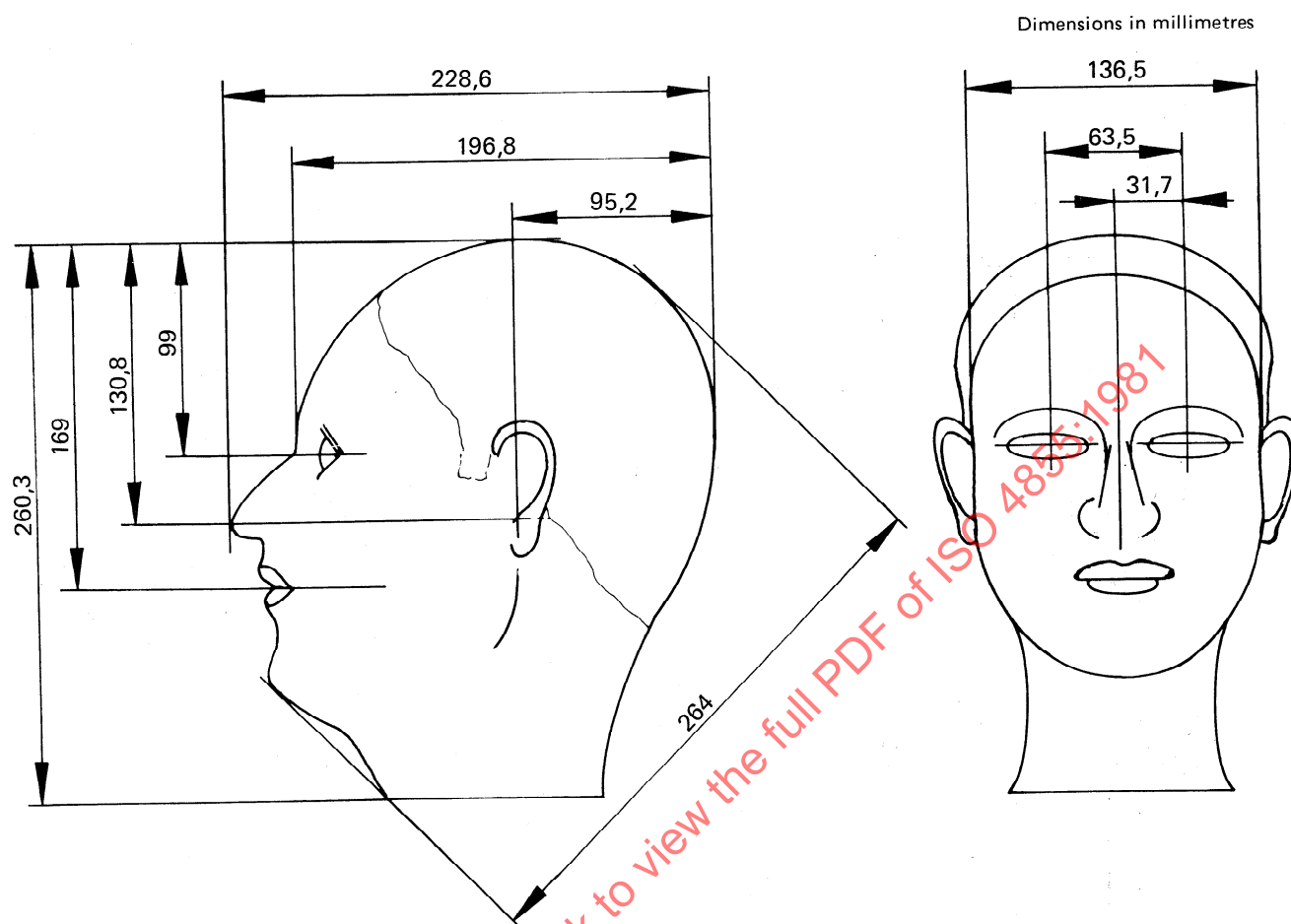
Figure 3 — Example of head-form for test for resistance to high-speed particles
