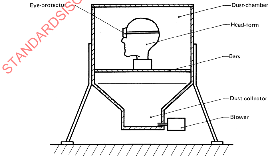
Figure 6 — Apparatus for test for protection against dust
