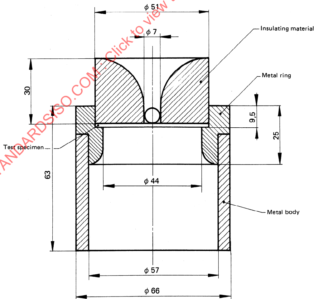
Figure 5 — Apparatus for testing resistance to penetration of hot solids
