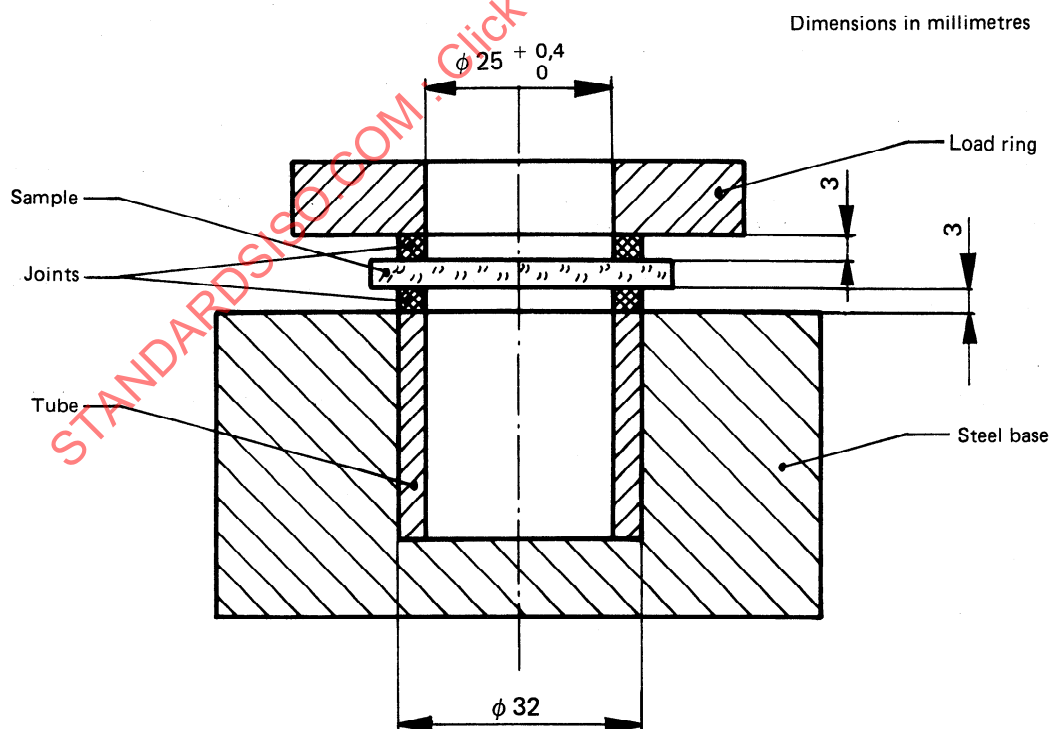
Figure 1 — Apparatus for test for robustness of unmounted oculars
