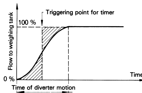
Figure 3 — Operational law of diverter
