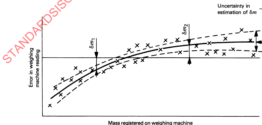
Figure 5 — Example of error distribution in calibration of weighing machine
