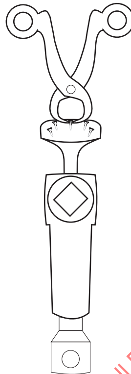
Figure 4 — Attachment to tensile testing machine by holding in the clamp
