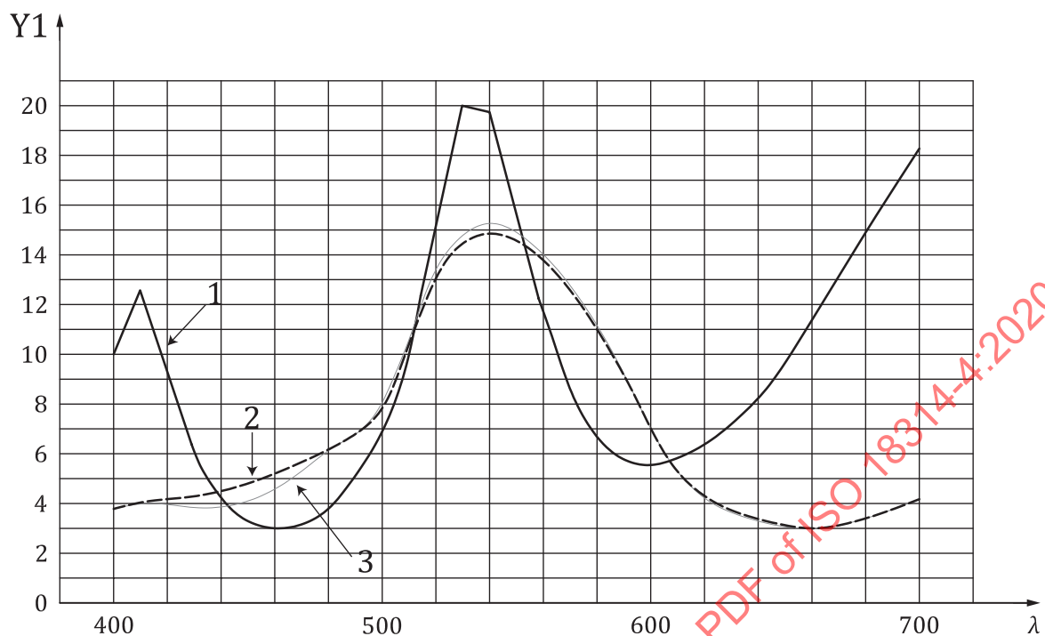
a) Reflectance functions of a standard, the sample and corrected reflectance function of the sample
