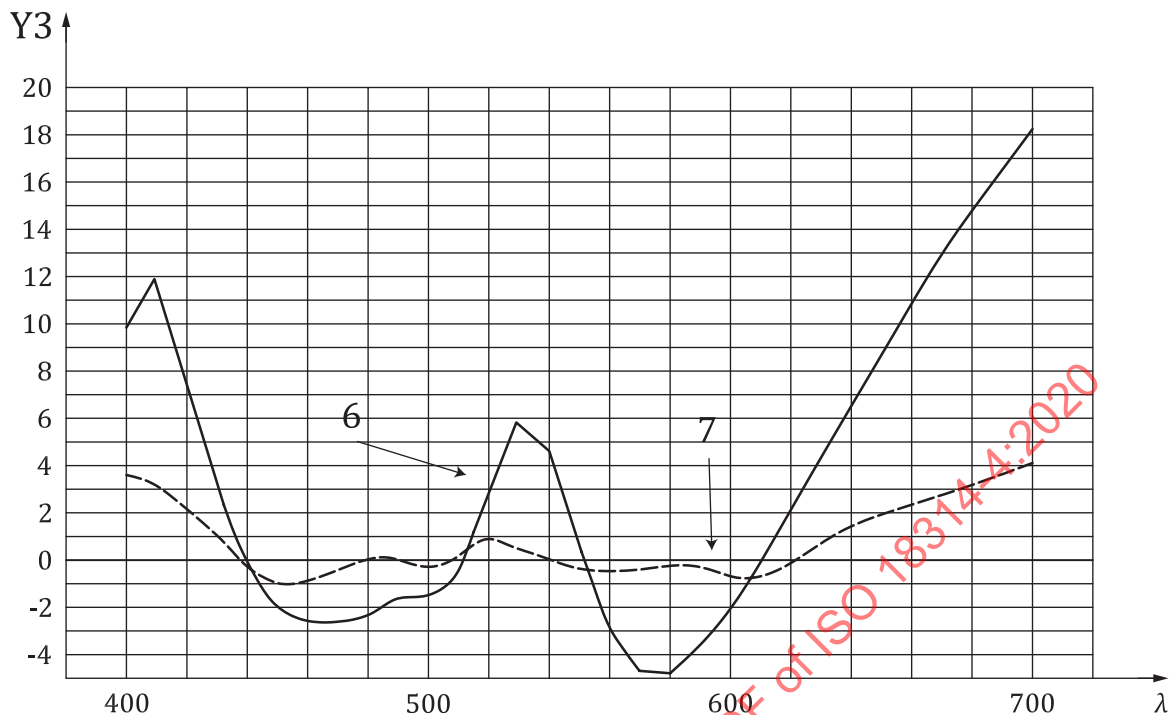
c) Metameric black values (residuals) of the reflectance functions of standard and sample for the decomposition for the reference illuminant D65
