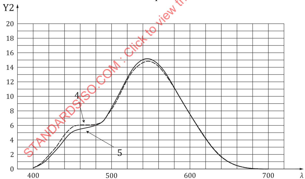
b) Fundamental reflectance function for the reference illuminant and corrected reflectance function of the sample Green-2 for the decomposition for the reference illuminant D65
