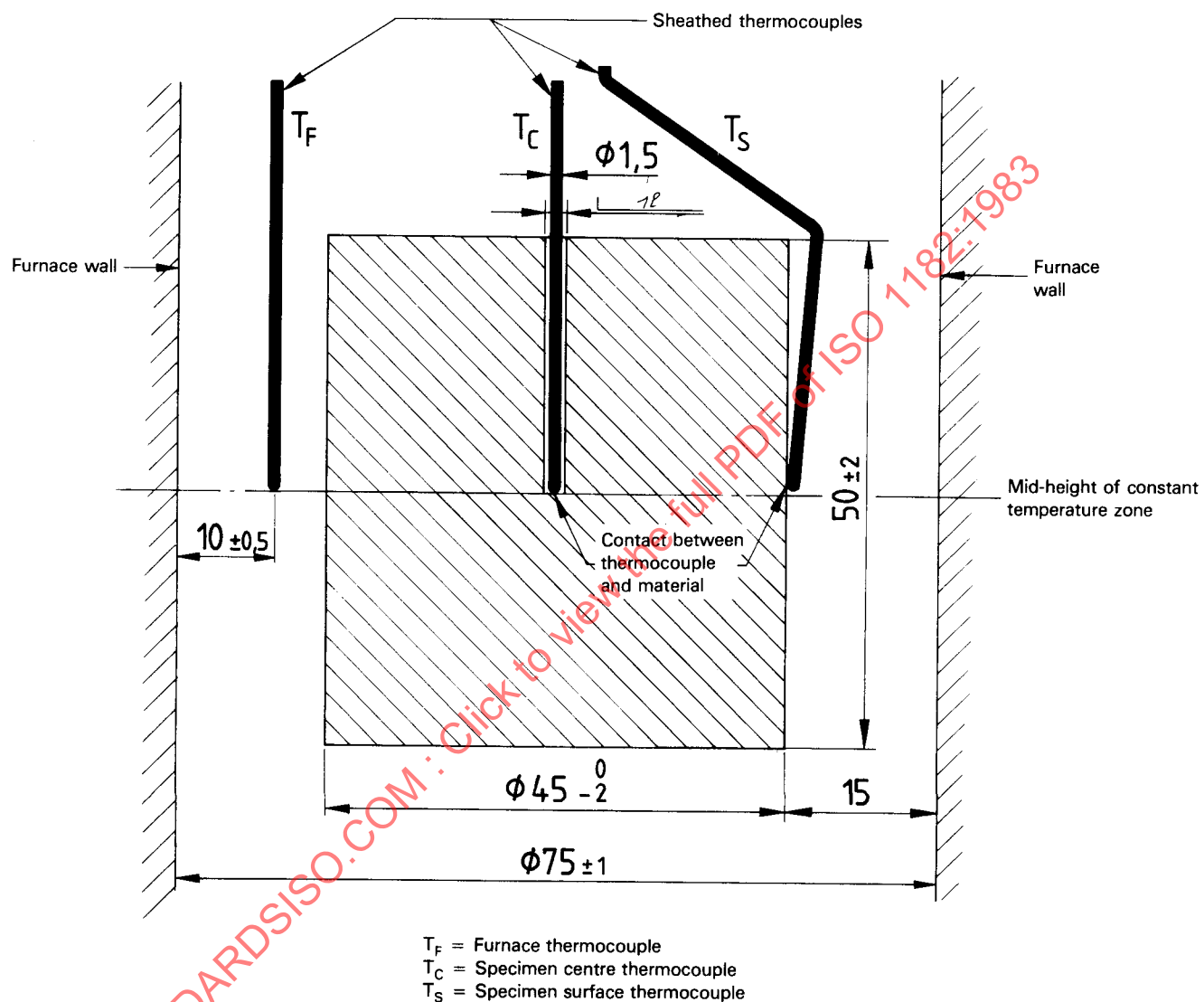
Figure 5 — Relative position of furnace, specimen and thermocouples
