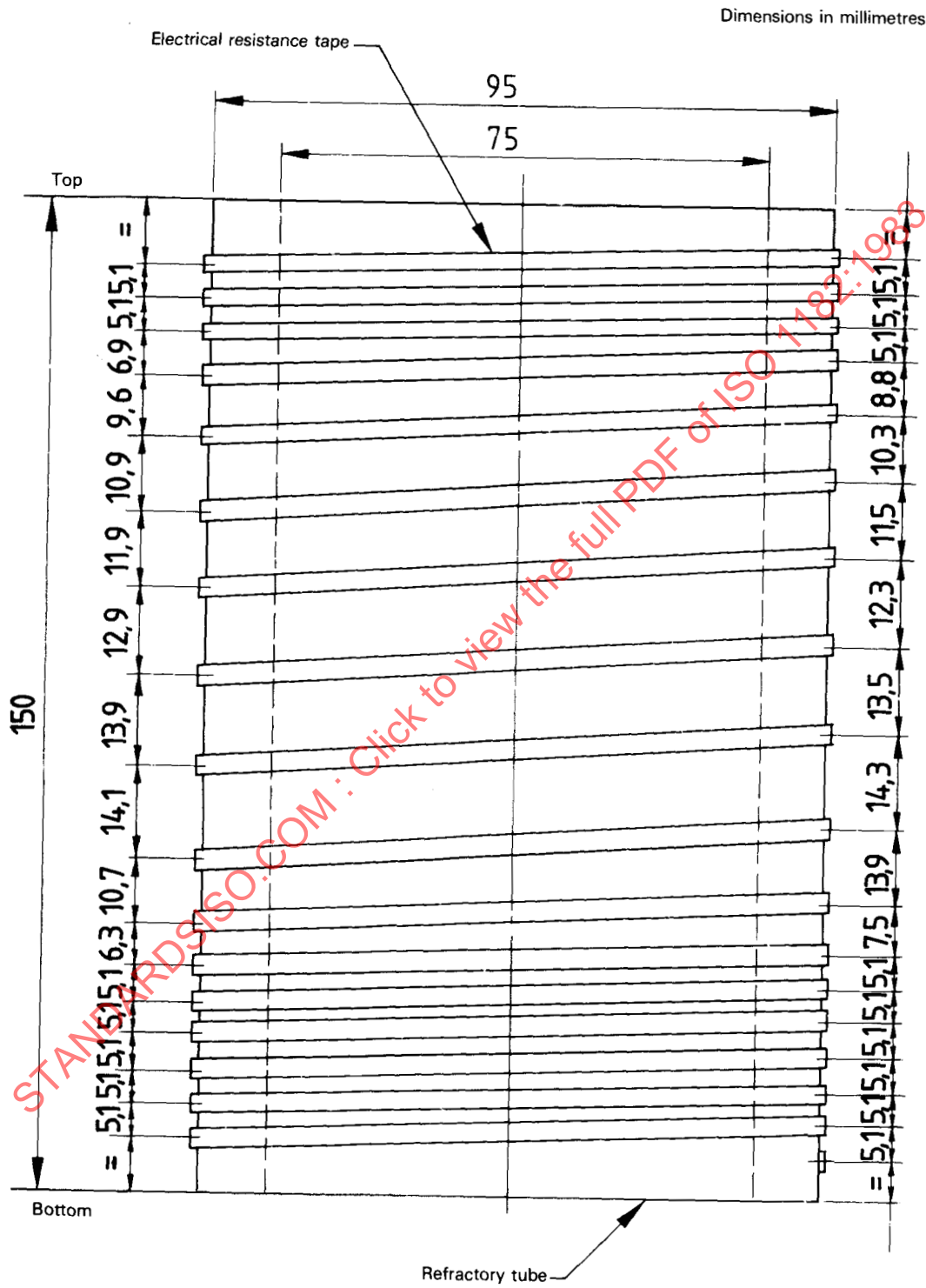
Figure 2 — Furnace windings
