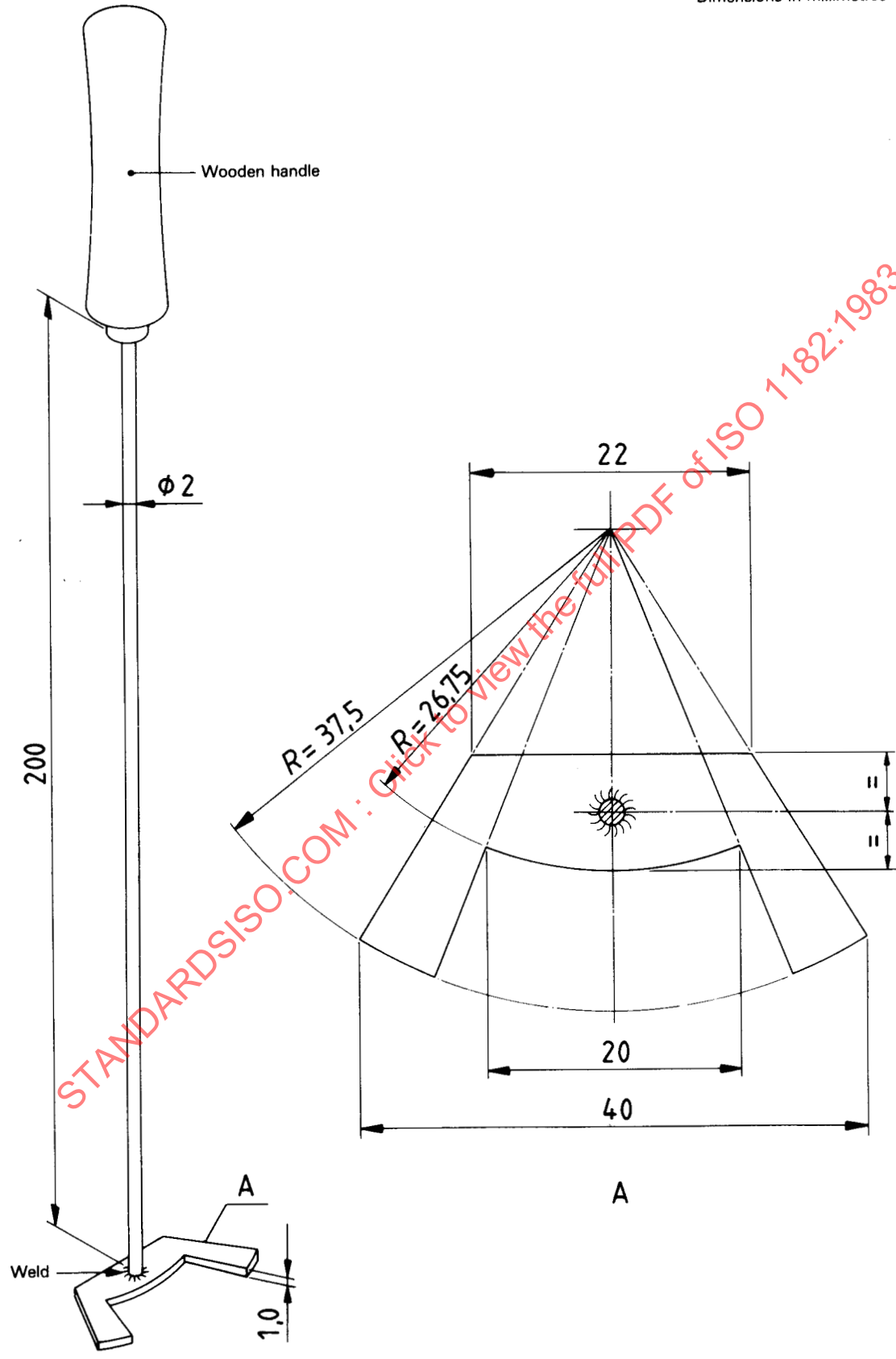
Figure 4 — Locating guide
