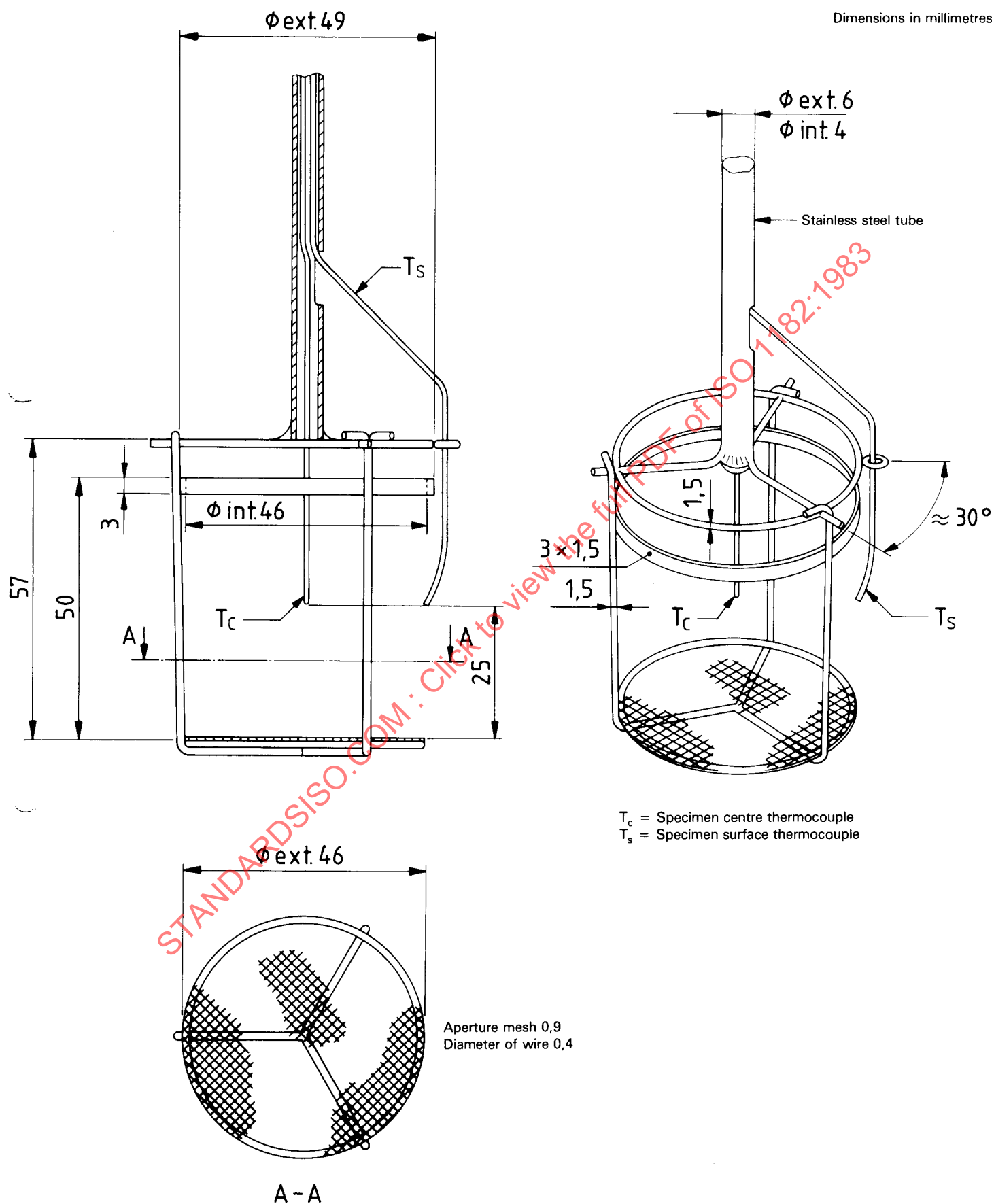
Figure 3 — Specimen holder
