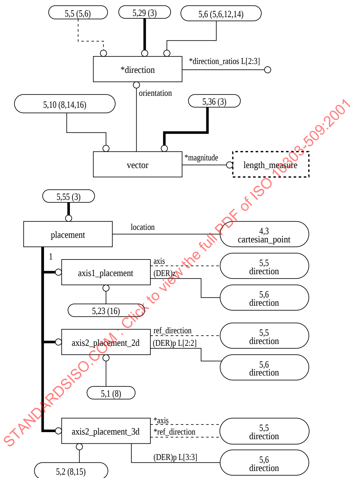
Figure C.5 – EXPRESS-G diagram 5 of 22
