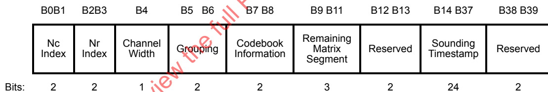
Figure 9-121d—CMMG MIMO Control field
