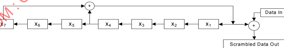
Figure 25-11—Scrambler
