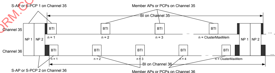
Figure 10-58b—Example of decentralized clusters for two APs or PCPs of a synchronization pair
