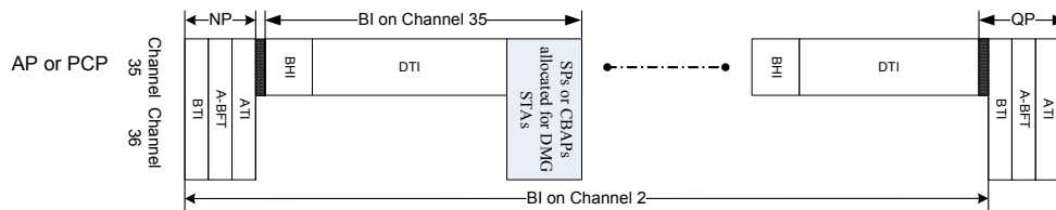
Figure 10-112—SPs or CBAPs allocated for DMG STAs on channel 2 with beacon intervals starting on channel 35
