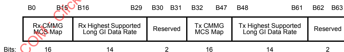
Figure 9-589dj—Supported CMMG MCS and NSS Set field
