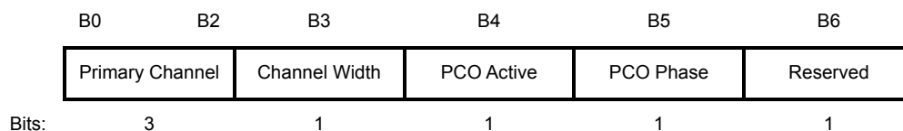
Figure 9-589do—CMMG Operation Information field
