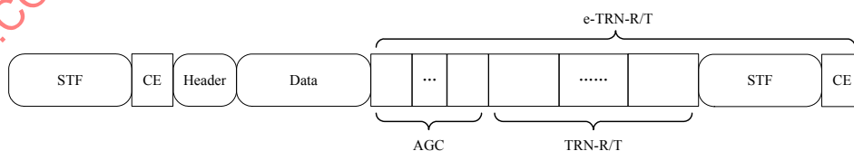
Figure 24-9—BRP packet structure (CDMG STAs)
