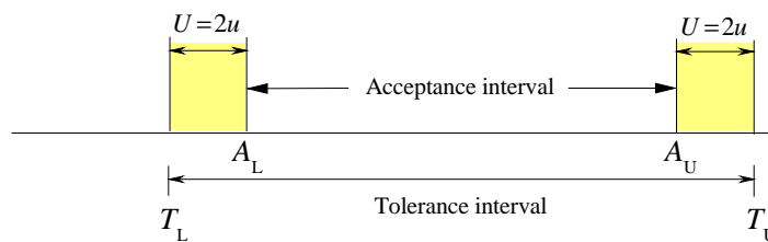
Figure 10 – Two-sided acceptance interval created by reducing the tolerance interval on either side by the k = 2 expanded uncertainty U = 2u . This is the default decision rule established in ISO 14253-1 [21].
